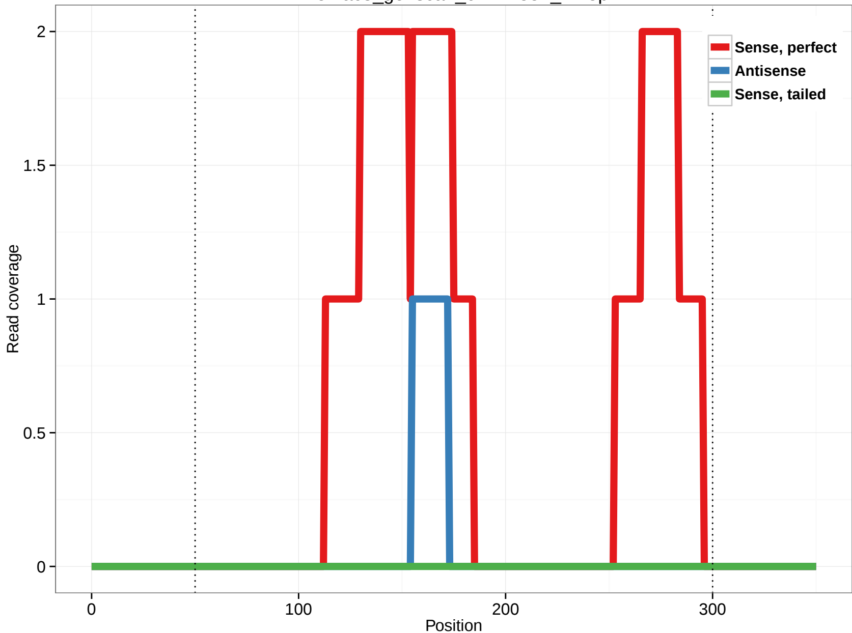
rheMac3_genscan_chr2.1551_14.5p
