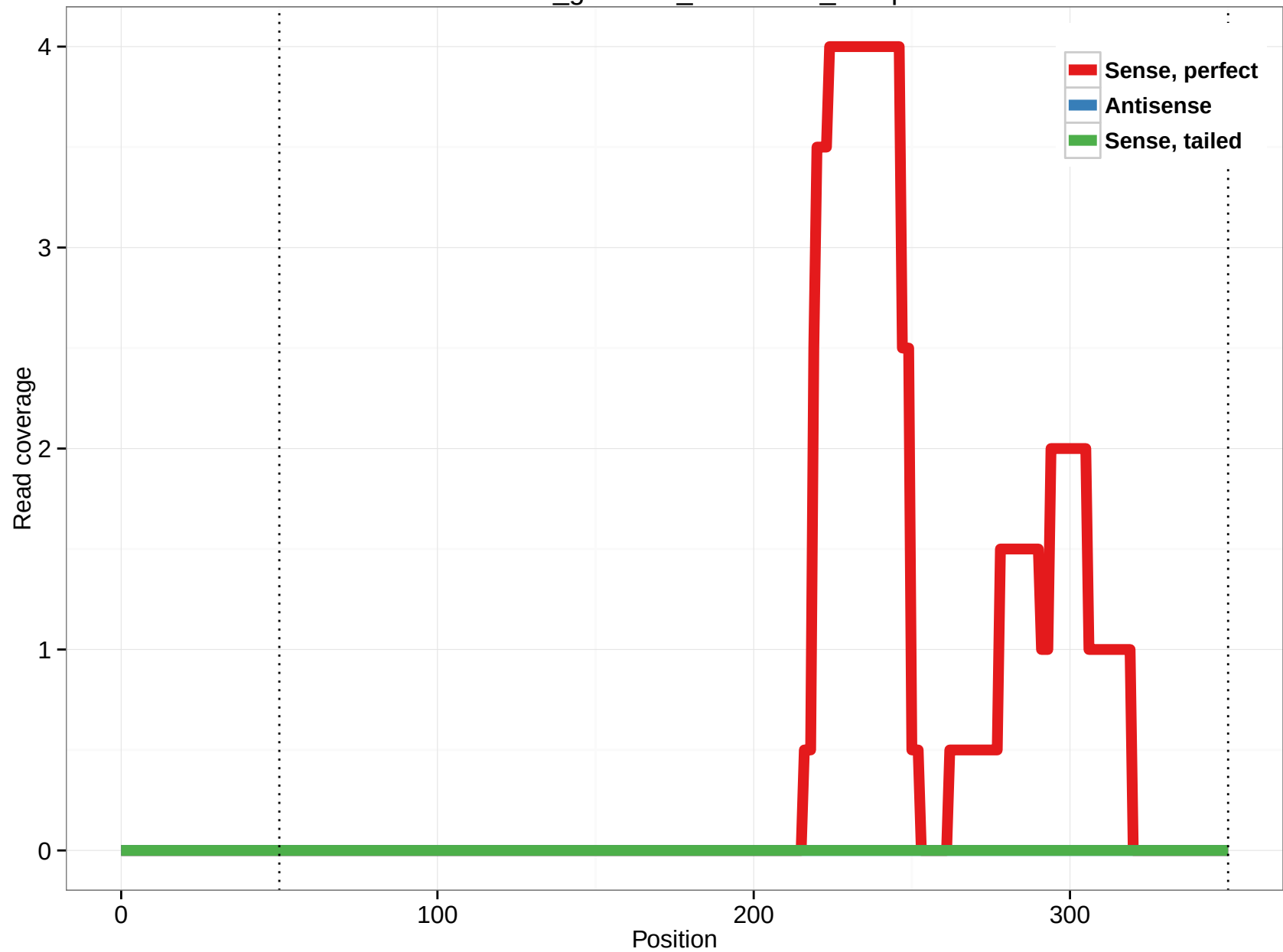
rheMac3_genscan_chr2.1480_11.5p
