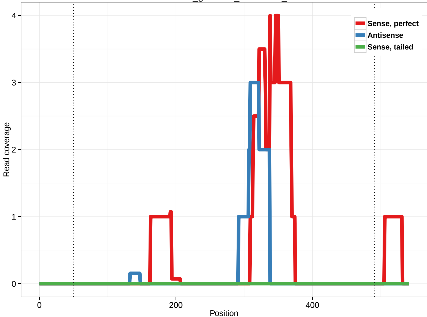
rheMac3_genscan_chr2.1472_3
