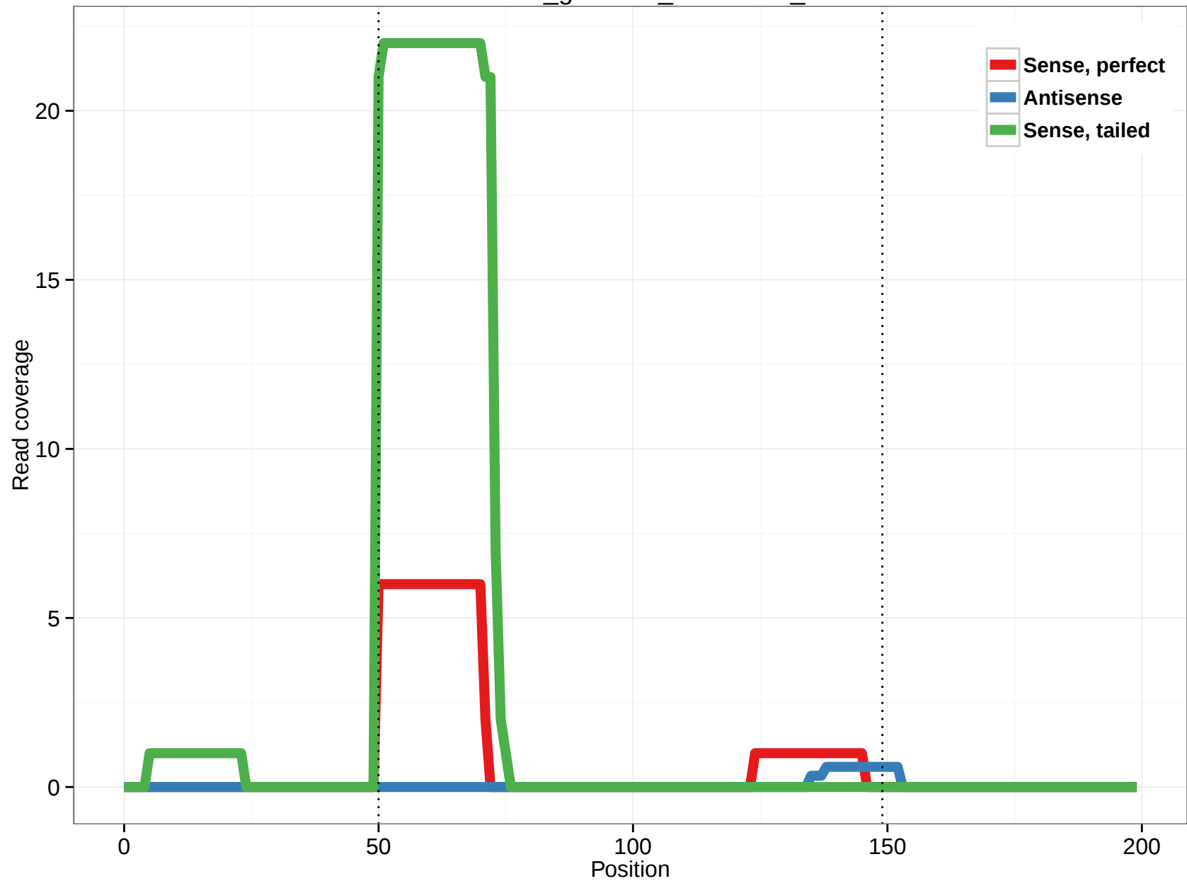
rheMac3_genscan_chr2.1425_4
