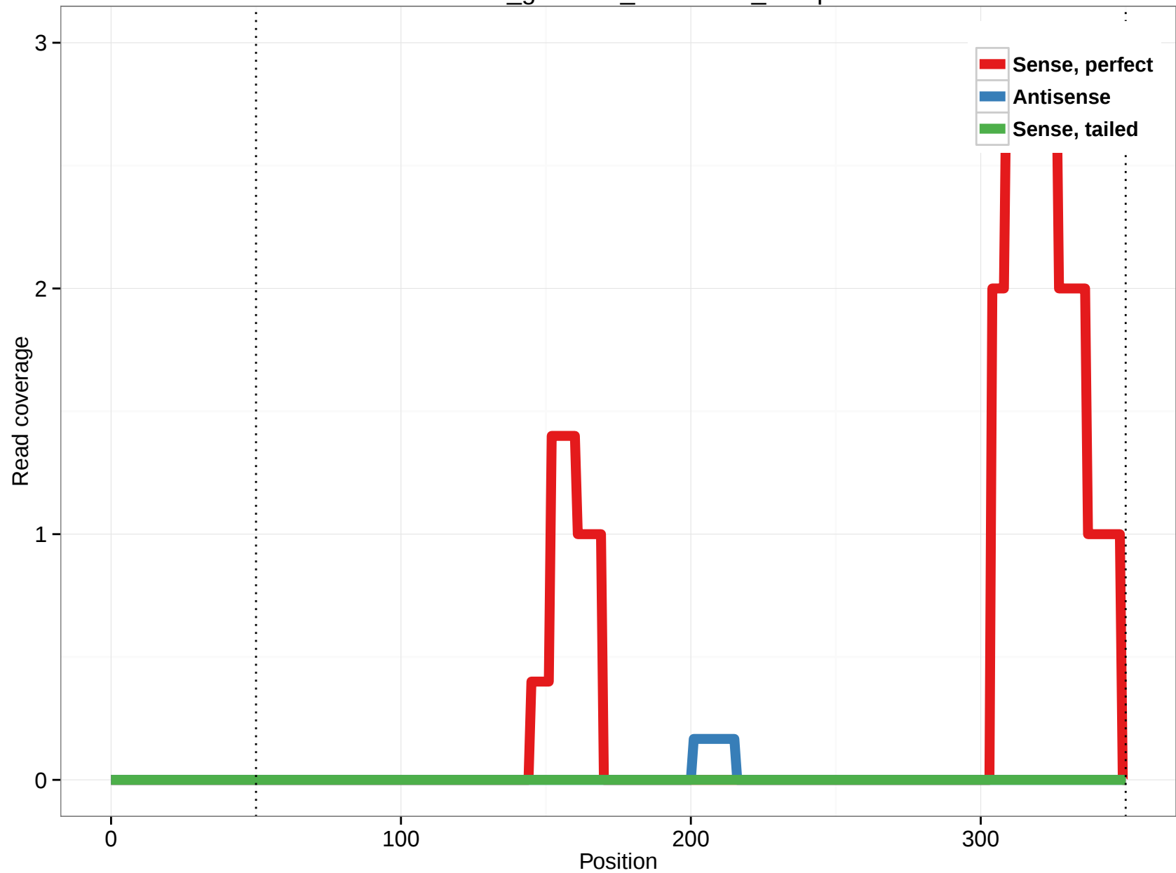
rheMac3_genscan_chr2.1423_16.5p
