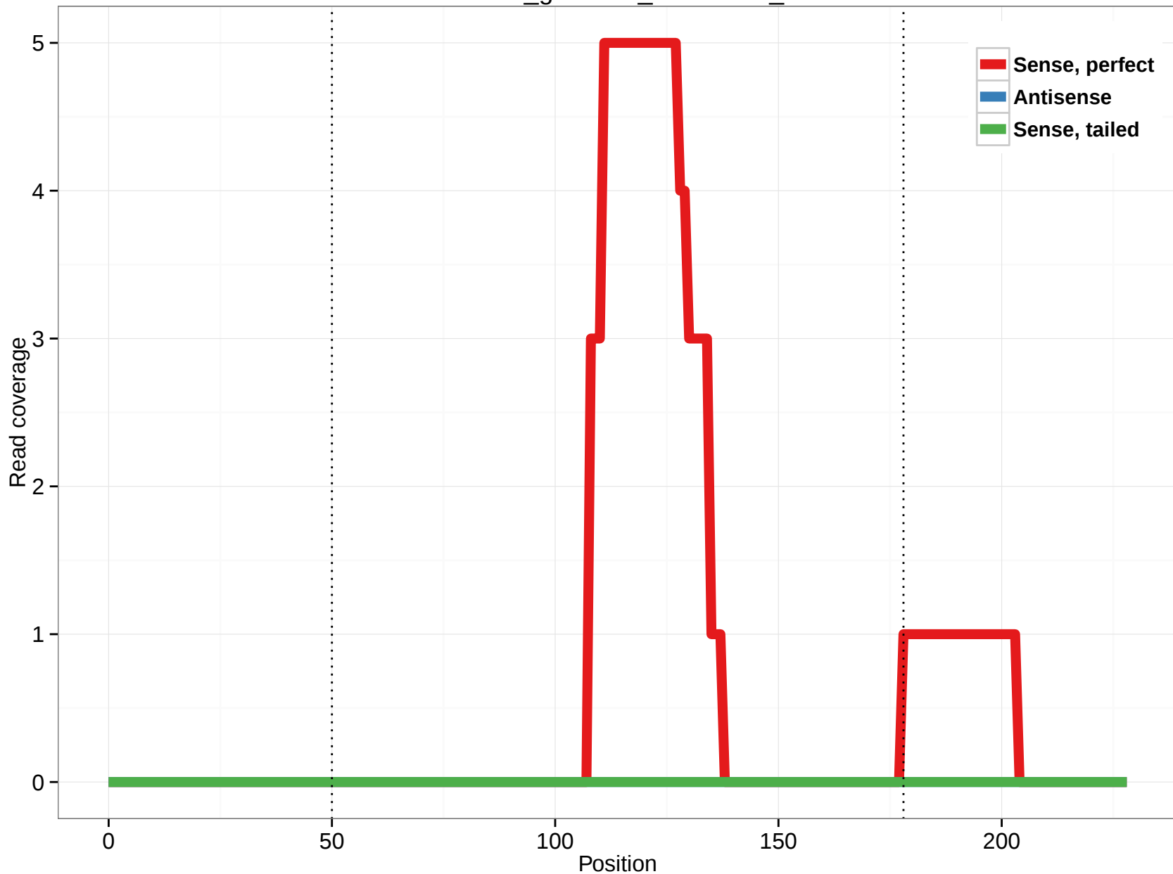
rheMac3_genscan_chr2.1395_13
