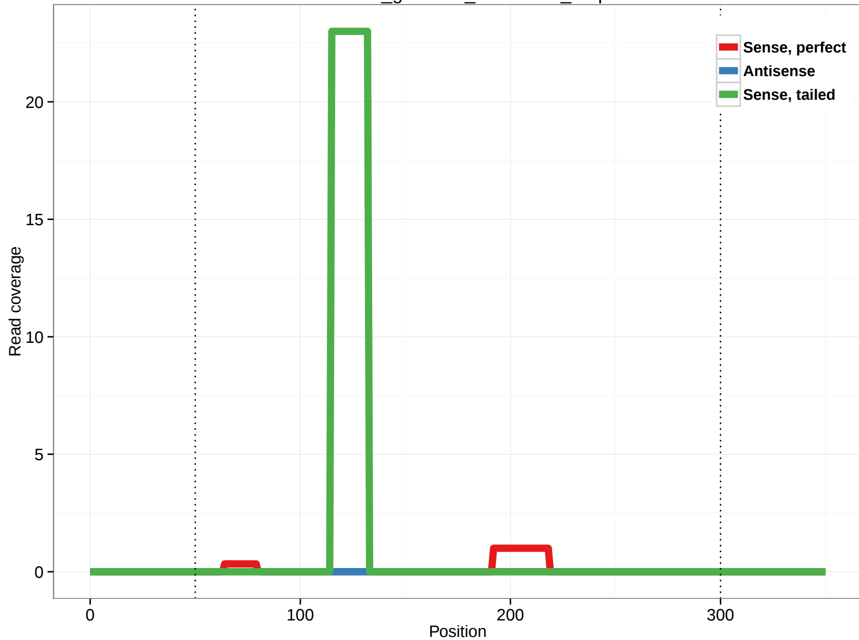
rheMac3_genscan_chr2.1309_2.3p
