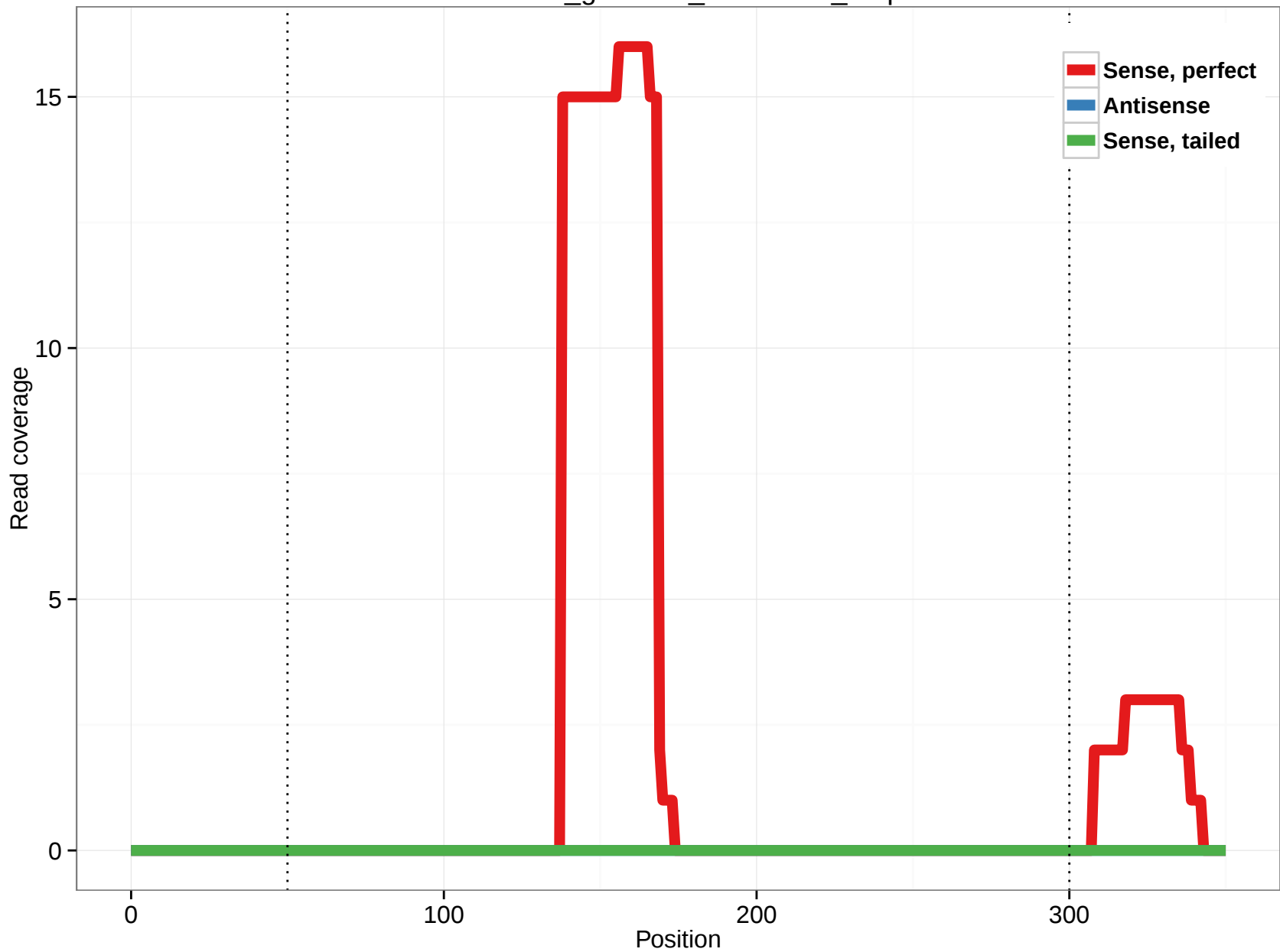
rheMac3_genscan_chr2.1278_8.3p
