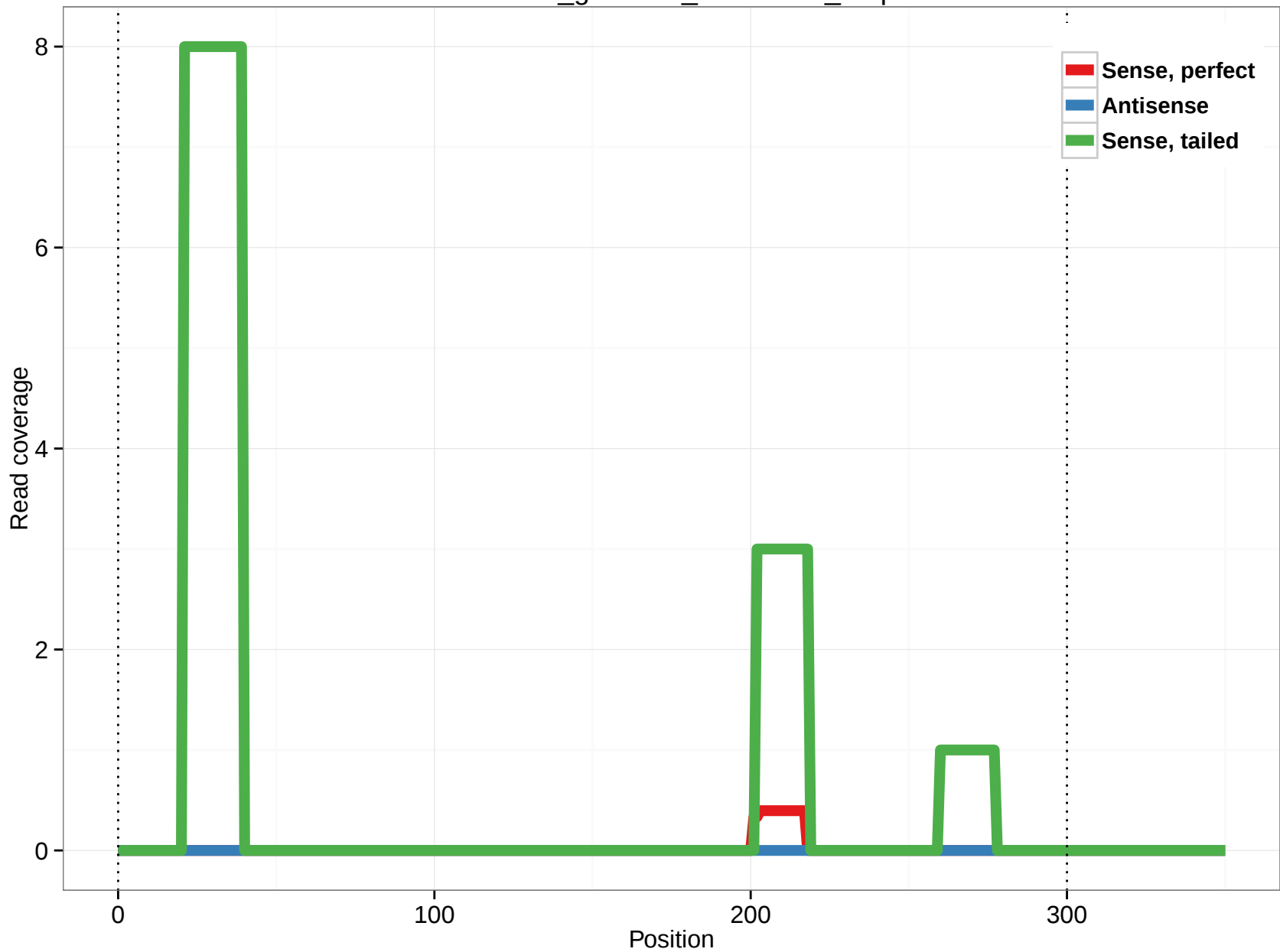
rheMac3_genscan_chr2.1251_2.3p
