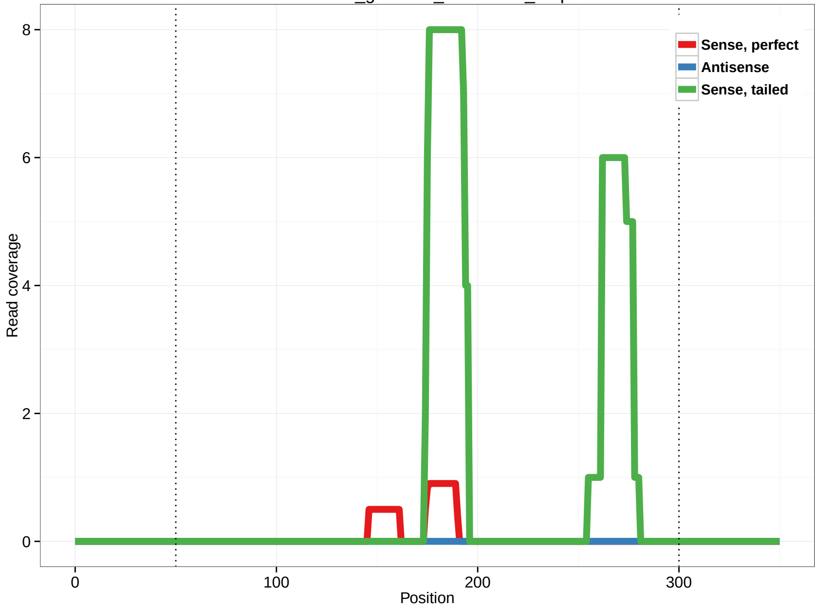
rheMac3_genscan_chr2.1248_4.3p
