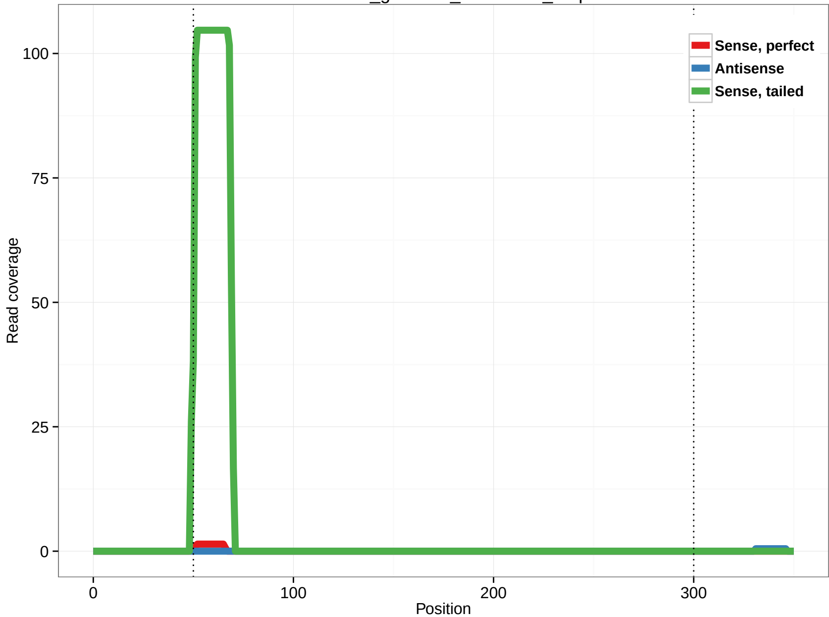
rheMac3_genscan_chr2.1220_5.3p
