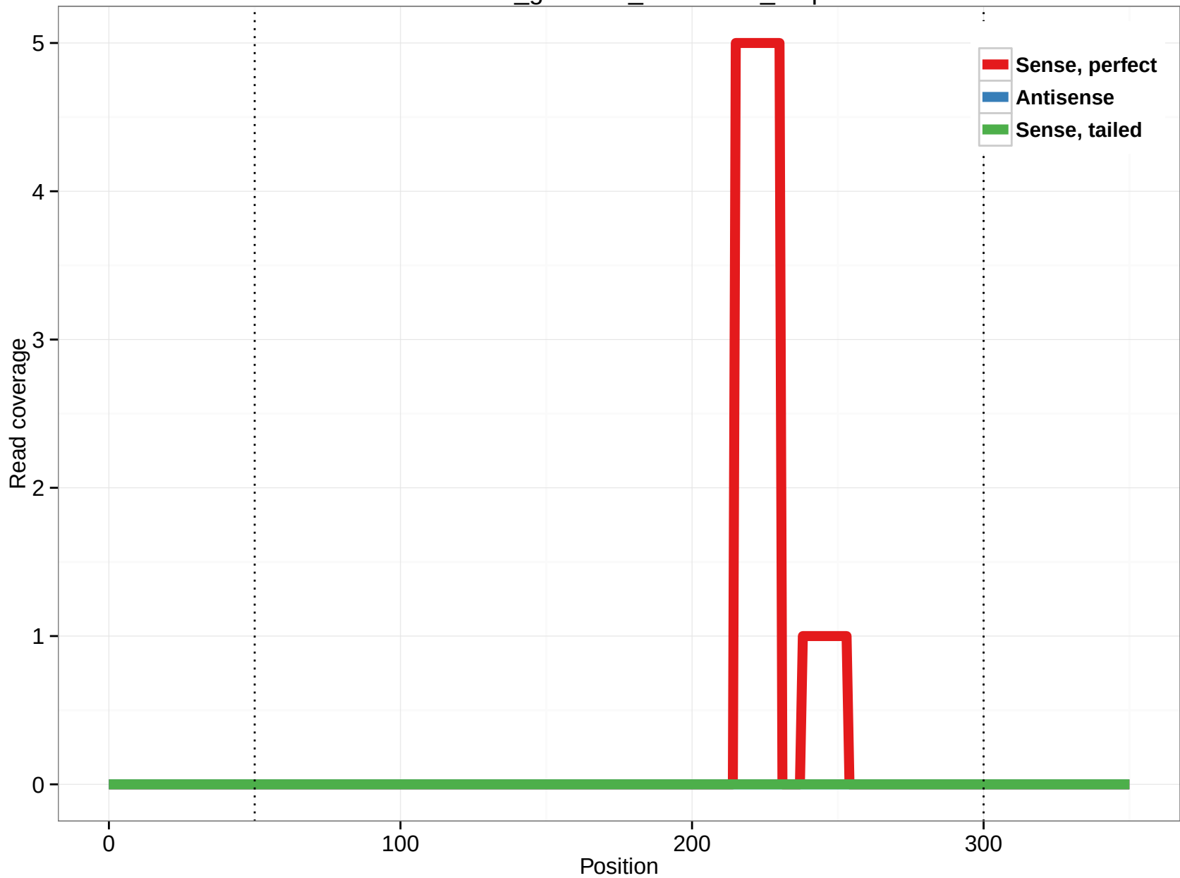
rheMac3_genscan_chr2.1148_2.3p
