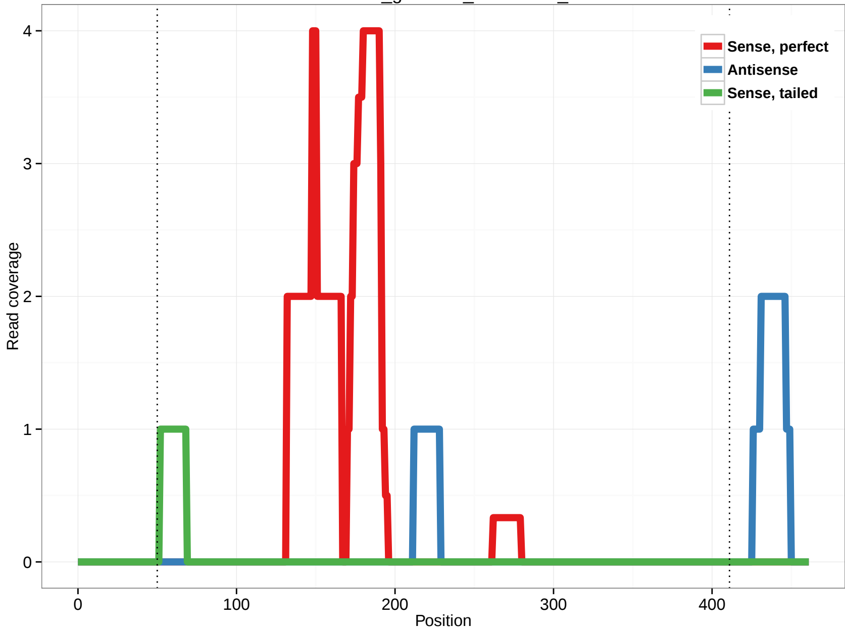
rheMac3_genscan_chr2.1119_3
