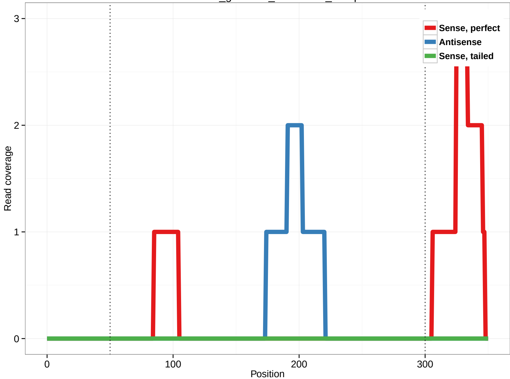
rheMac3_genscan_chr2.1082_23.3p
