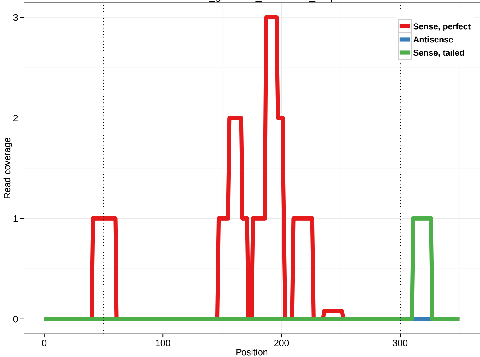
rheMac3_genscan_chr2.1063_2.5p
