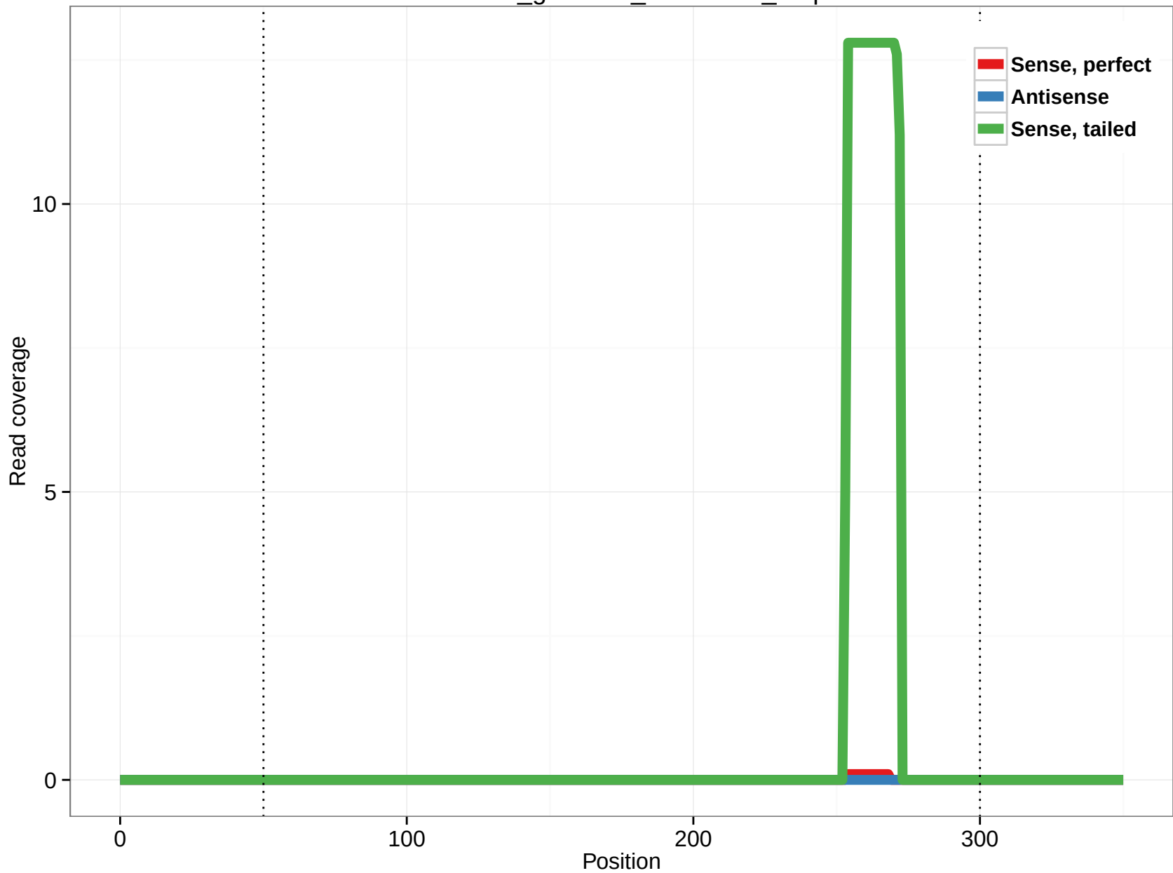
rheMac3_genscan_chr2.1060_0.3p
