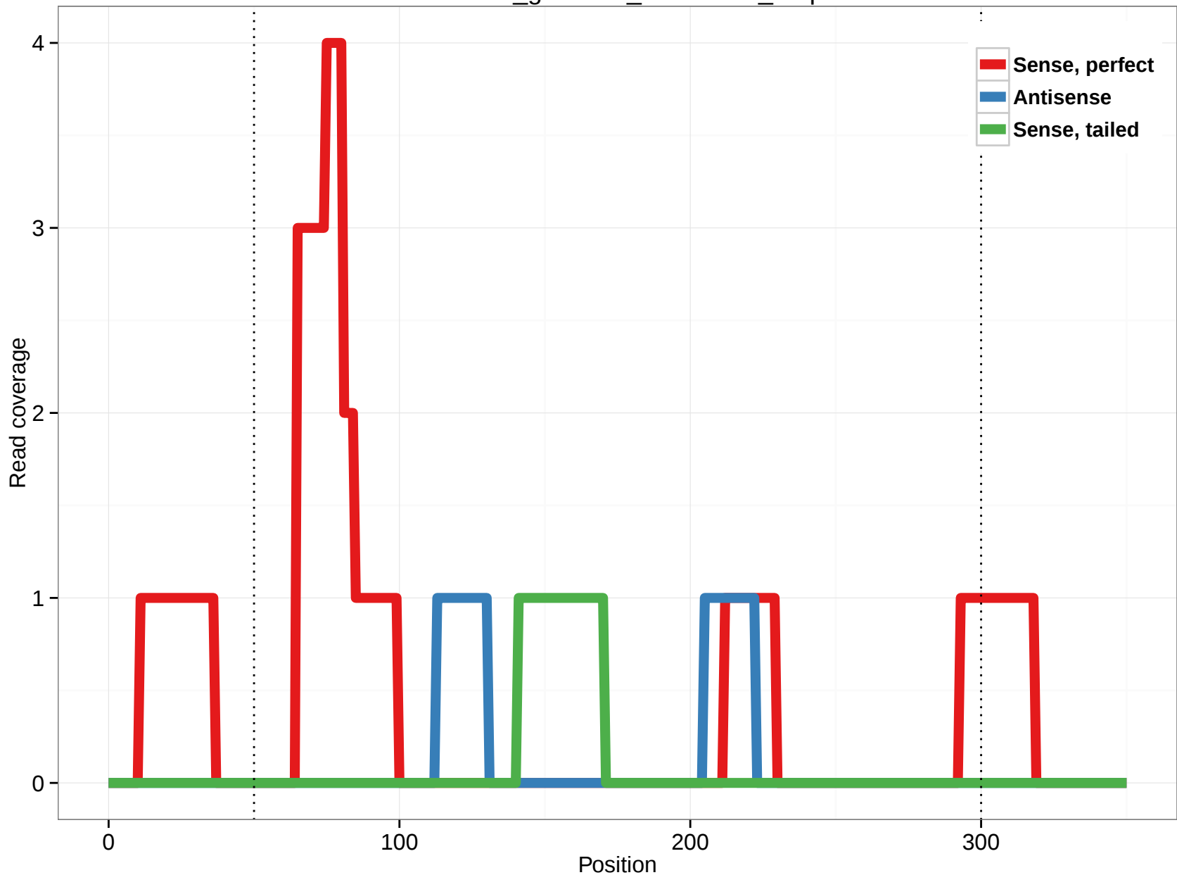
rheMac3_genscan_chr15.931_0.5p
