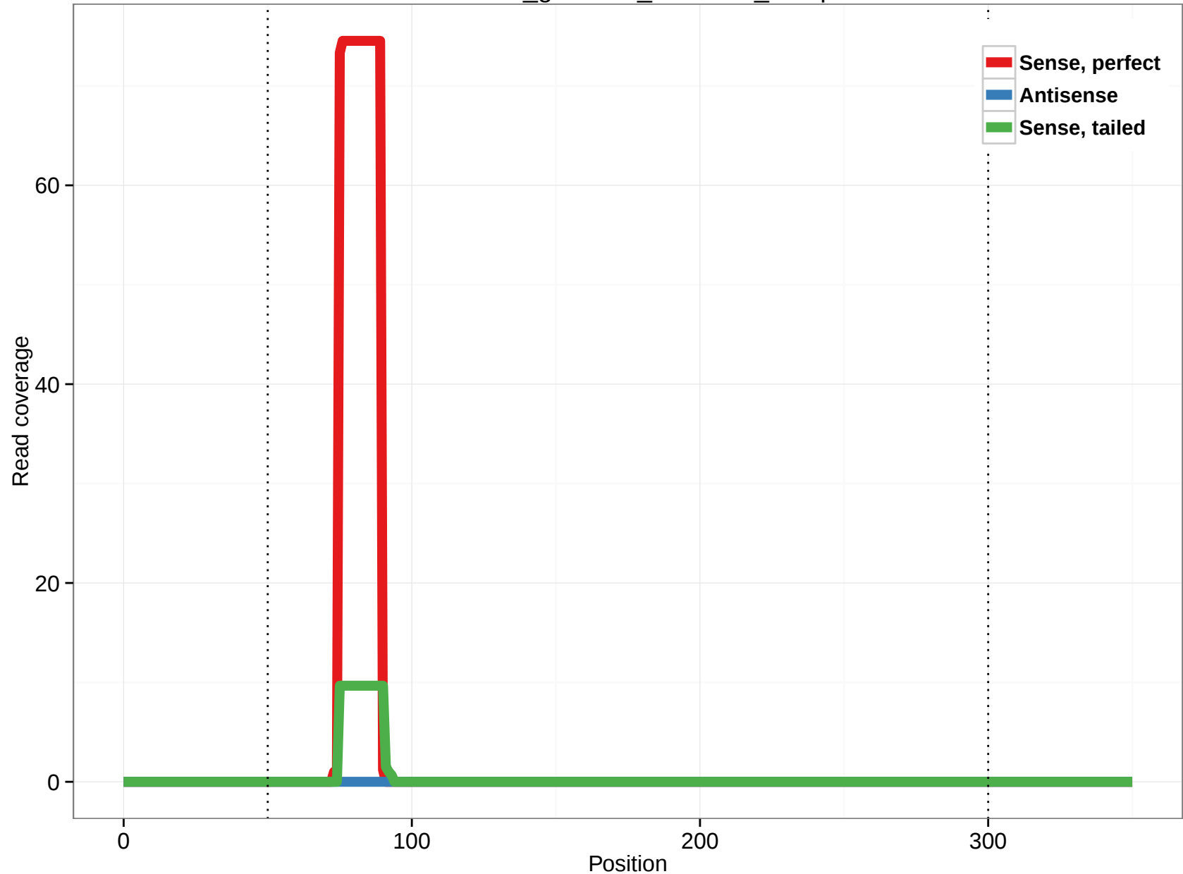
rheMac3_genscan_chr15.69_17.3p
