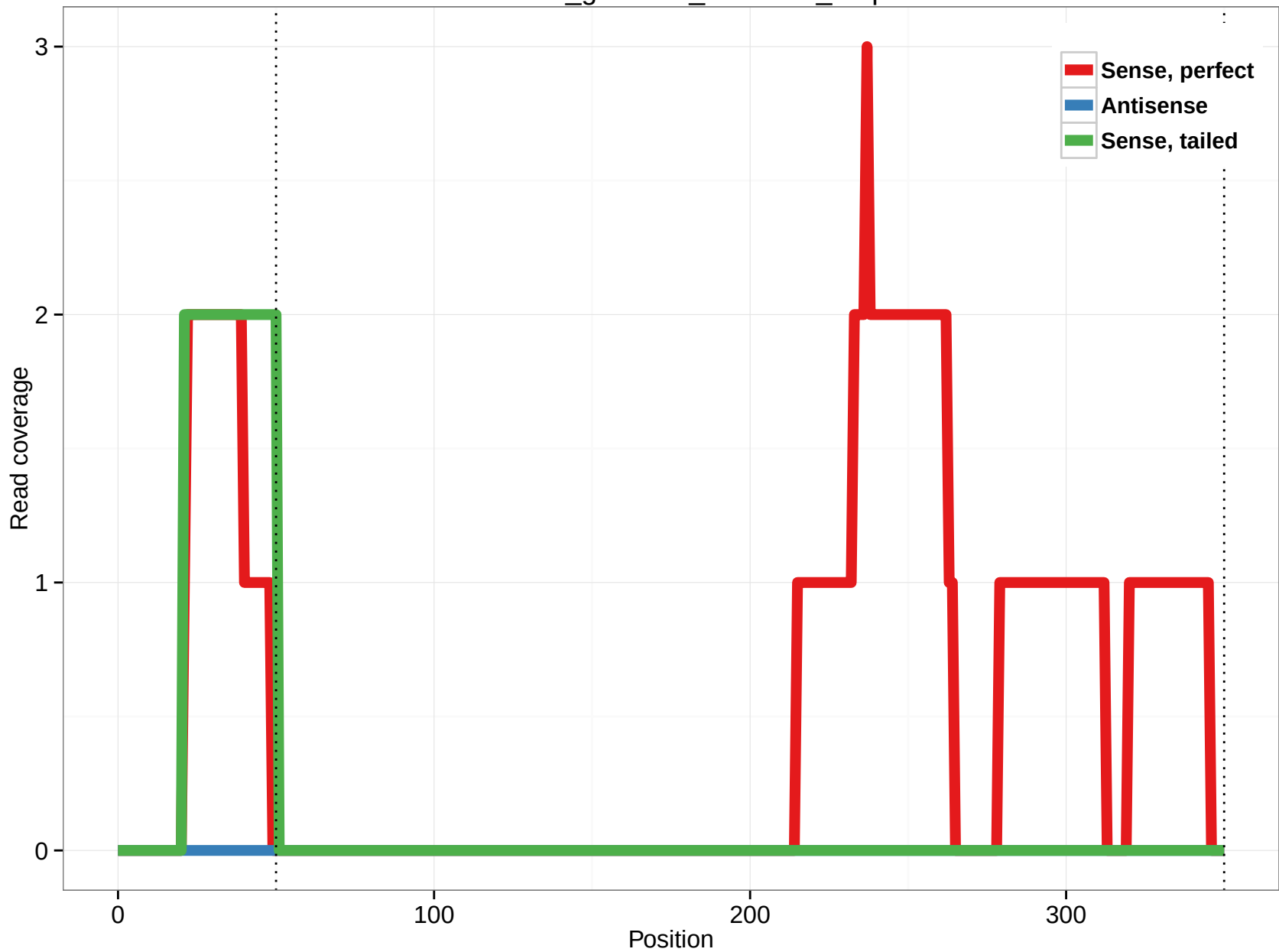
rheMac3_genscan_chr15.67_2.5p
