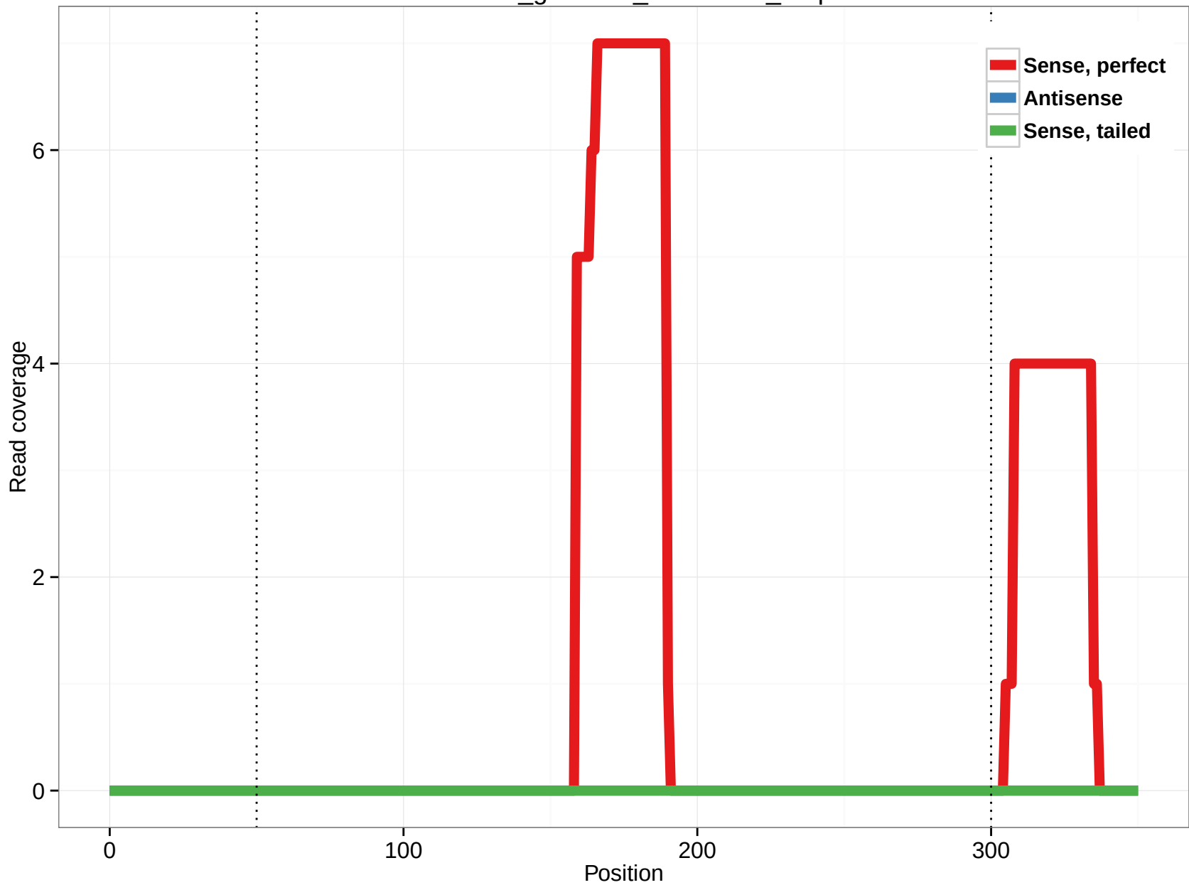
rheMac3_genscan_chr15.649_8.3p
