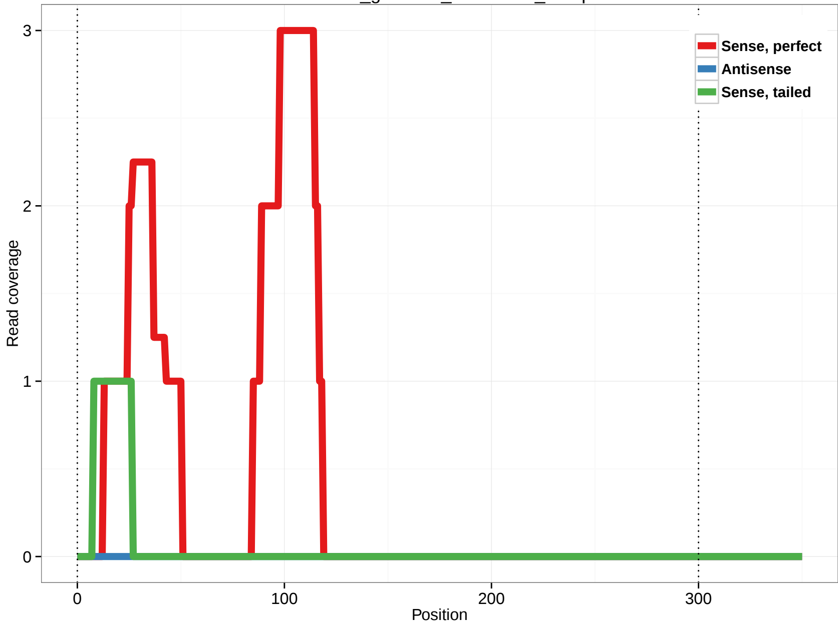
rheMac3_genscan_chr15.649_47.3p
