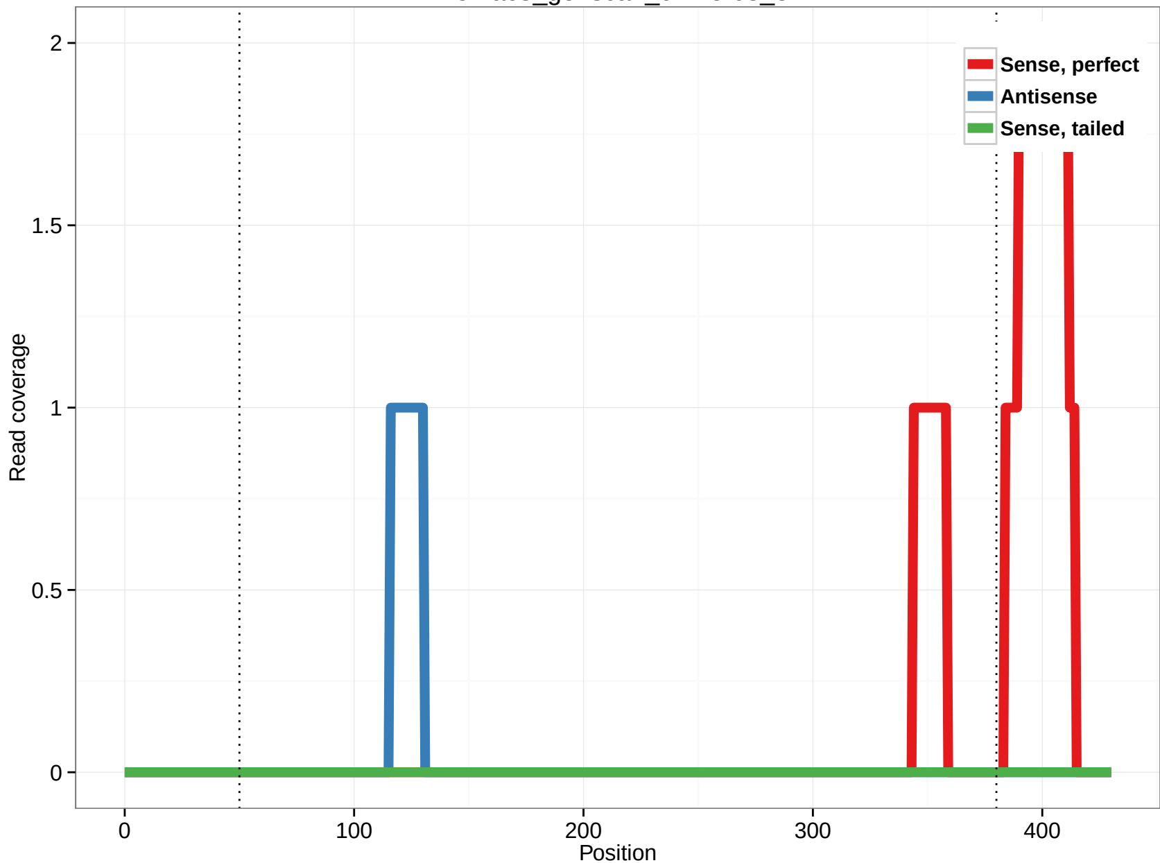
rheMac3_genscan_chr15.63_31
