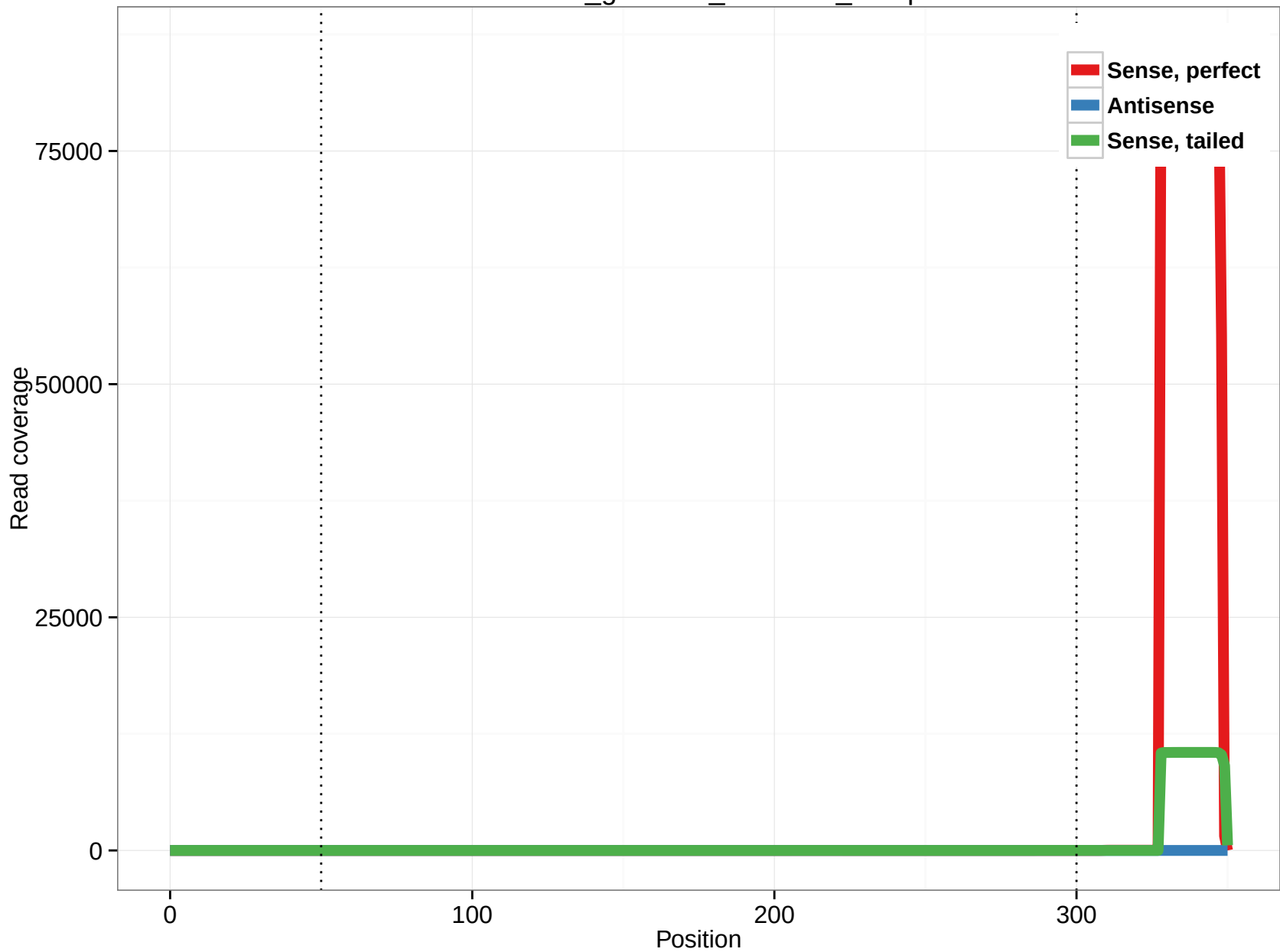
rheMac3_genscan_chr15.60_10.5p
