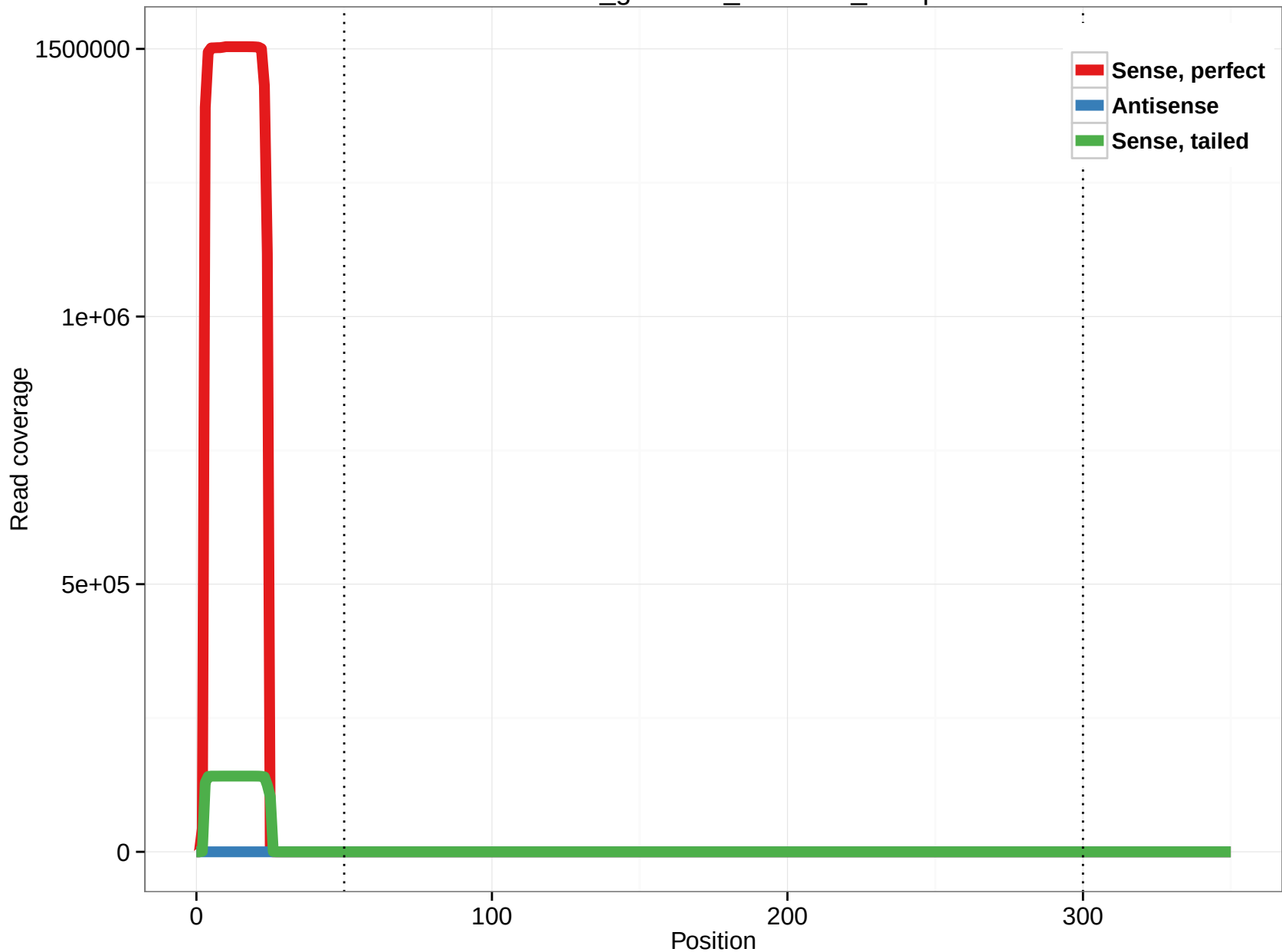
rheMac3_genscan_chr15.60_10.3p
