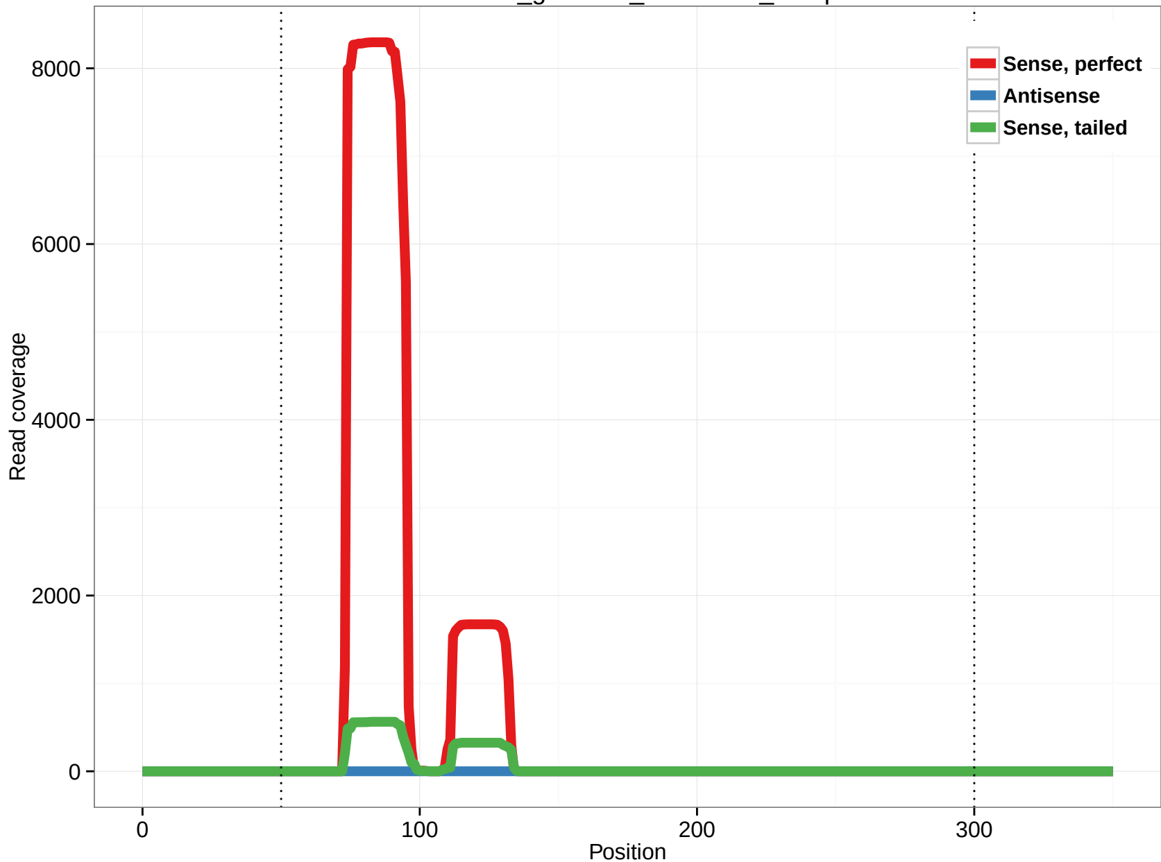
rheMac3_genscan_chr15.562_12.3p
