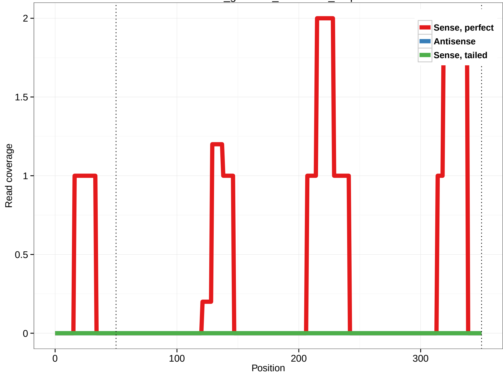
rheMac3_genscan_chr15.522_4.5p
