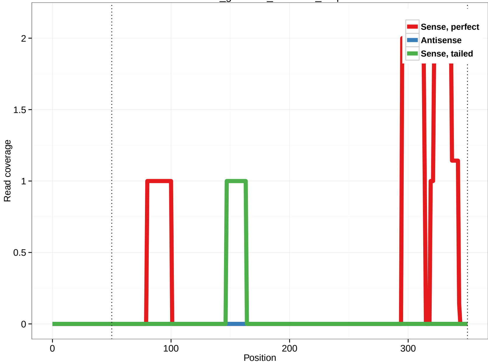
rheMac3_genscan_chr15.49_1.5p
