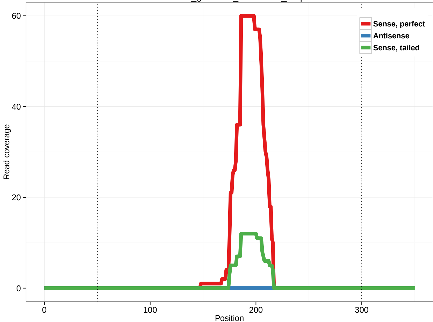
rheMac3_genscan_chr15.434_6.3p
