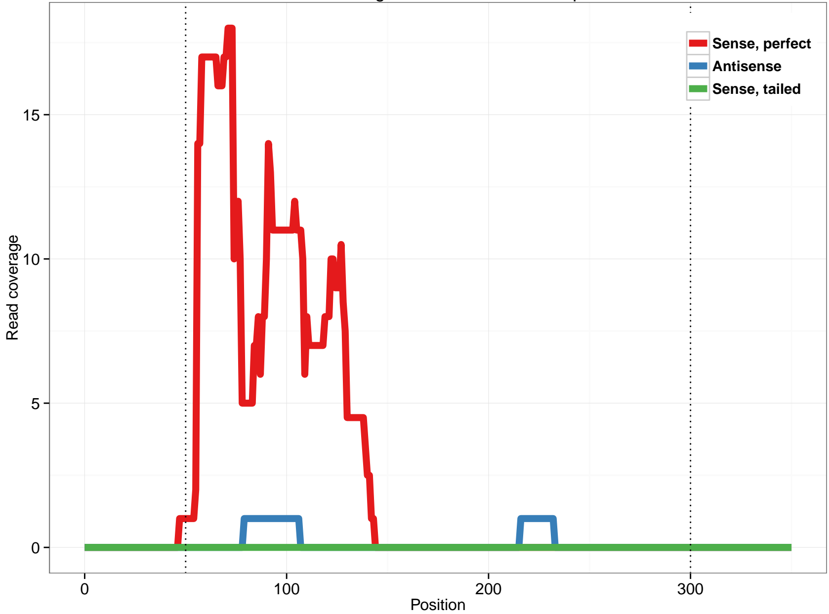
rheMac3_genscan_chr15.400_2.5p
