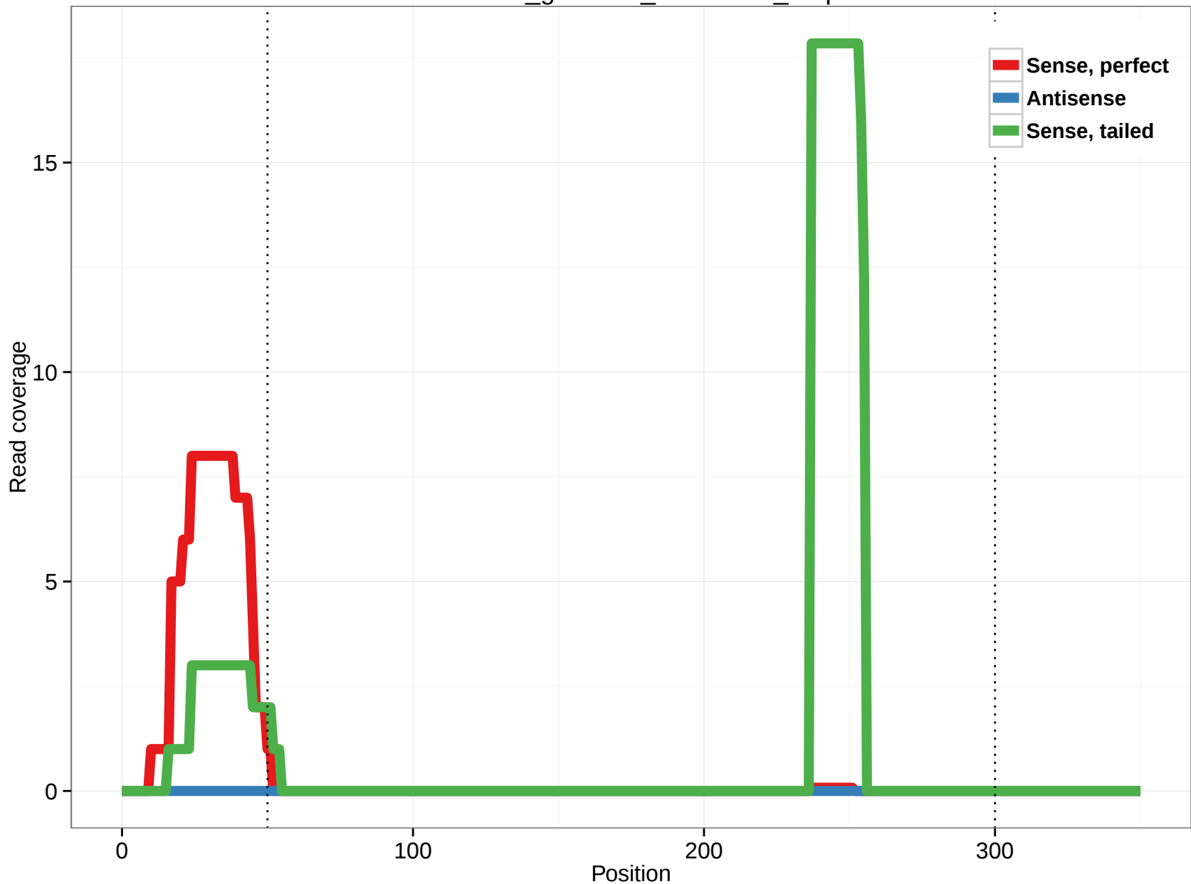
rheMac3_genscan_chr15.350_3.5p
