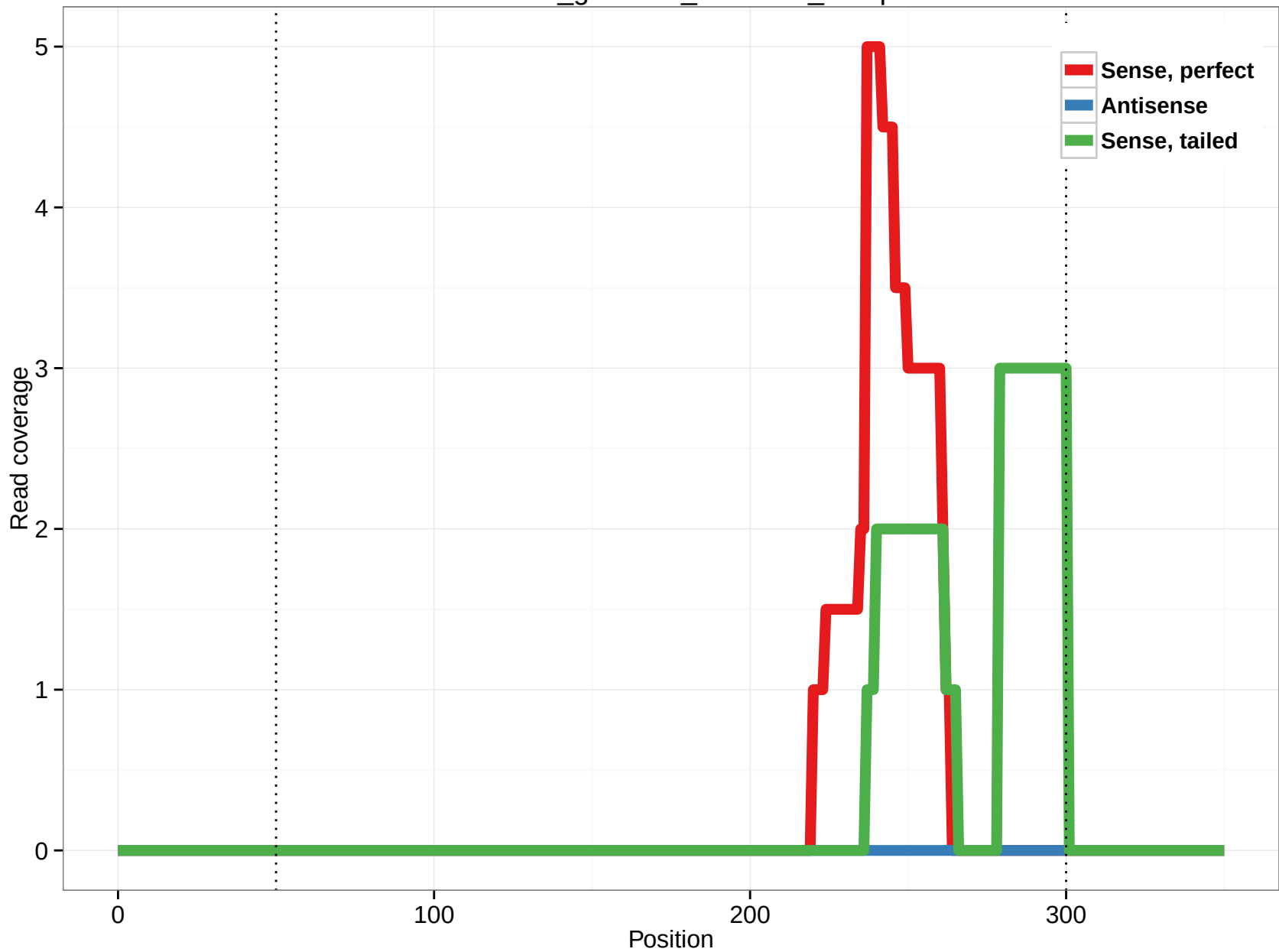
rheMac3_genscan_chr15.34_10.3p
