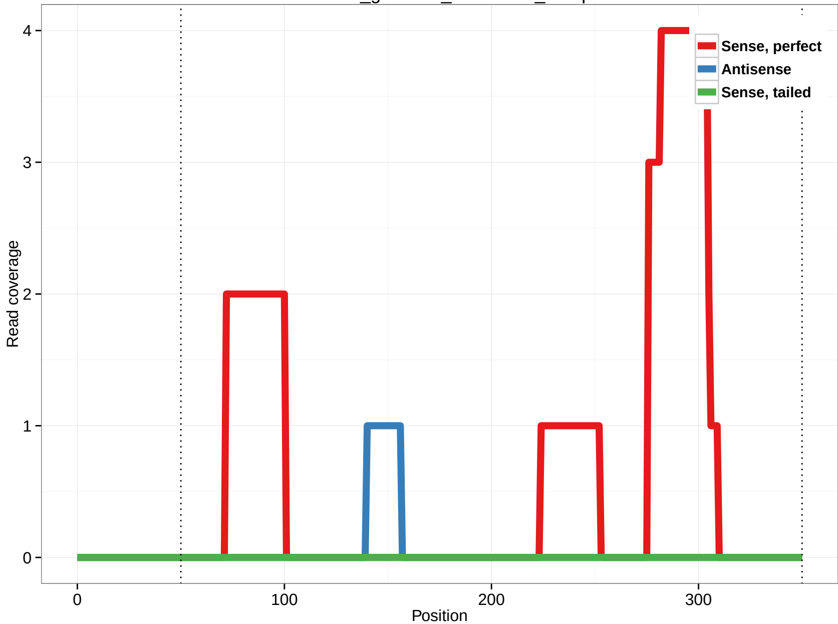
rheMac3_genscan_chr15.317_13.5p
