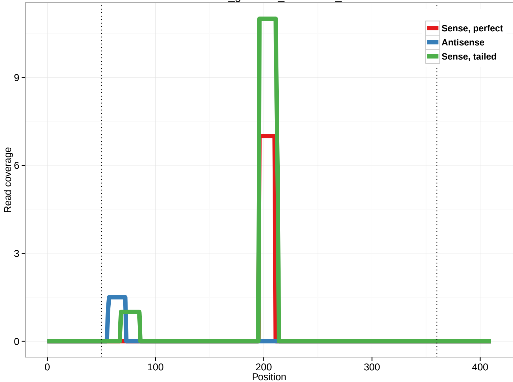
rheMac3_genscan_chr15.292_28
