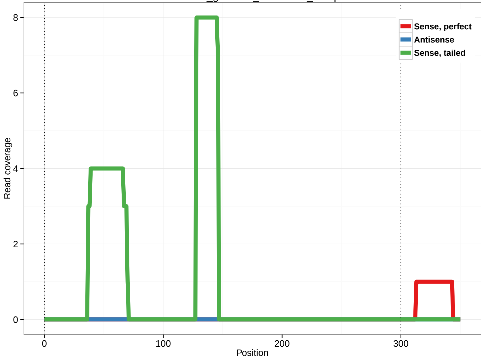
rheMac3_genscan_chr15.257_23.3p
