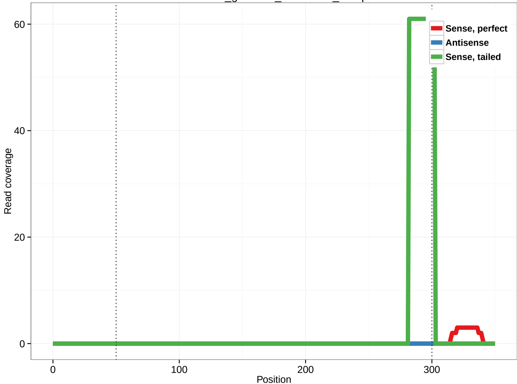
rheMac3_genscan_chr15.257_12.3p
