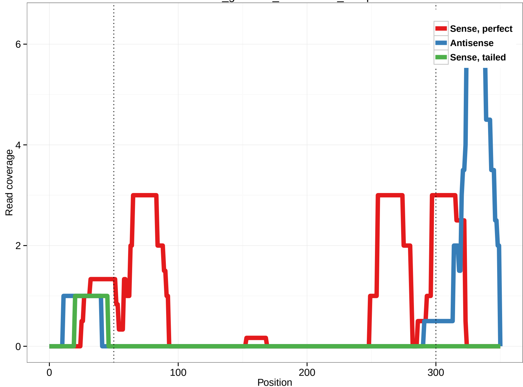
rheMac3_genscan_chr15.2247_11.3p
