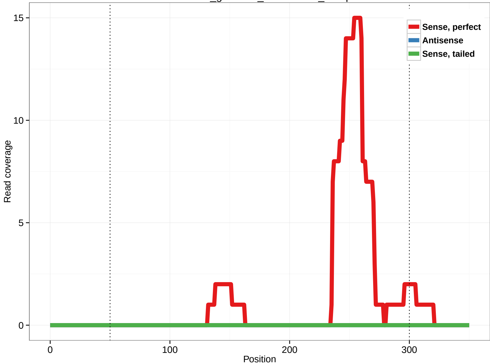
rheMac3_genscan_chr15.2167_12.5p
