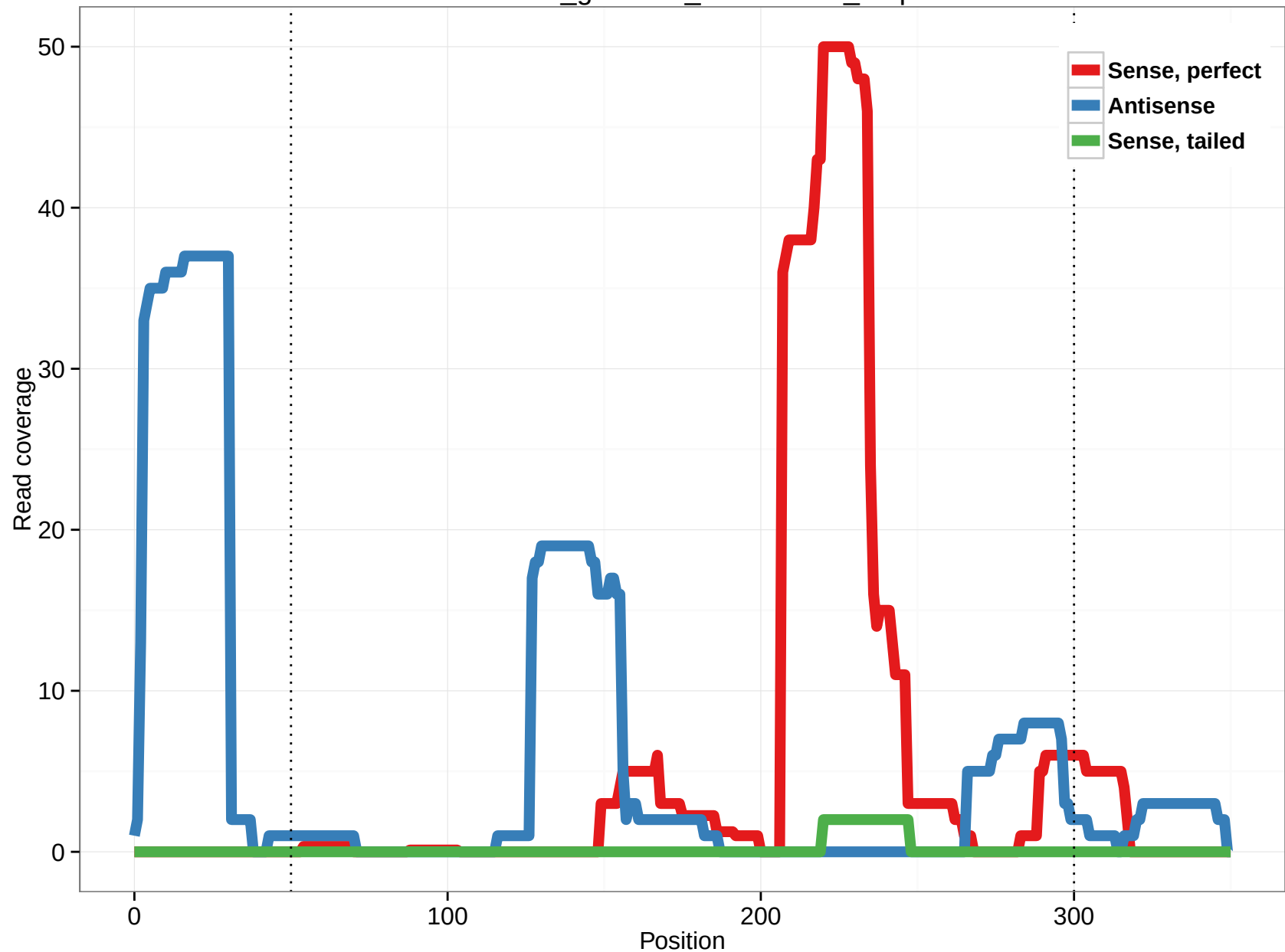
rheMac3_genscan_chr15.2091_6.5p
