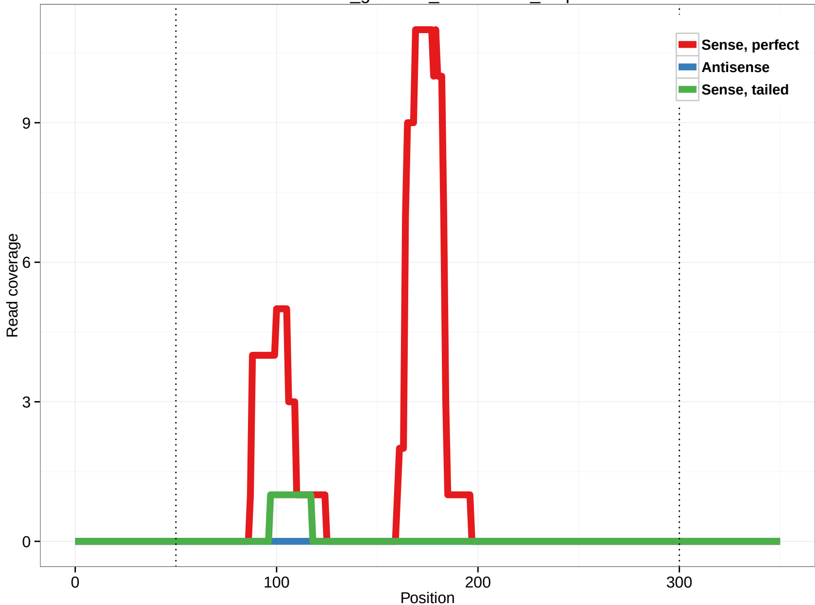
rheMac3_genscan_chr15.2033_1.5p
