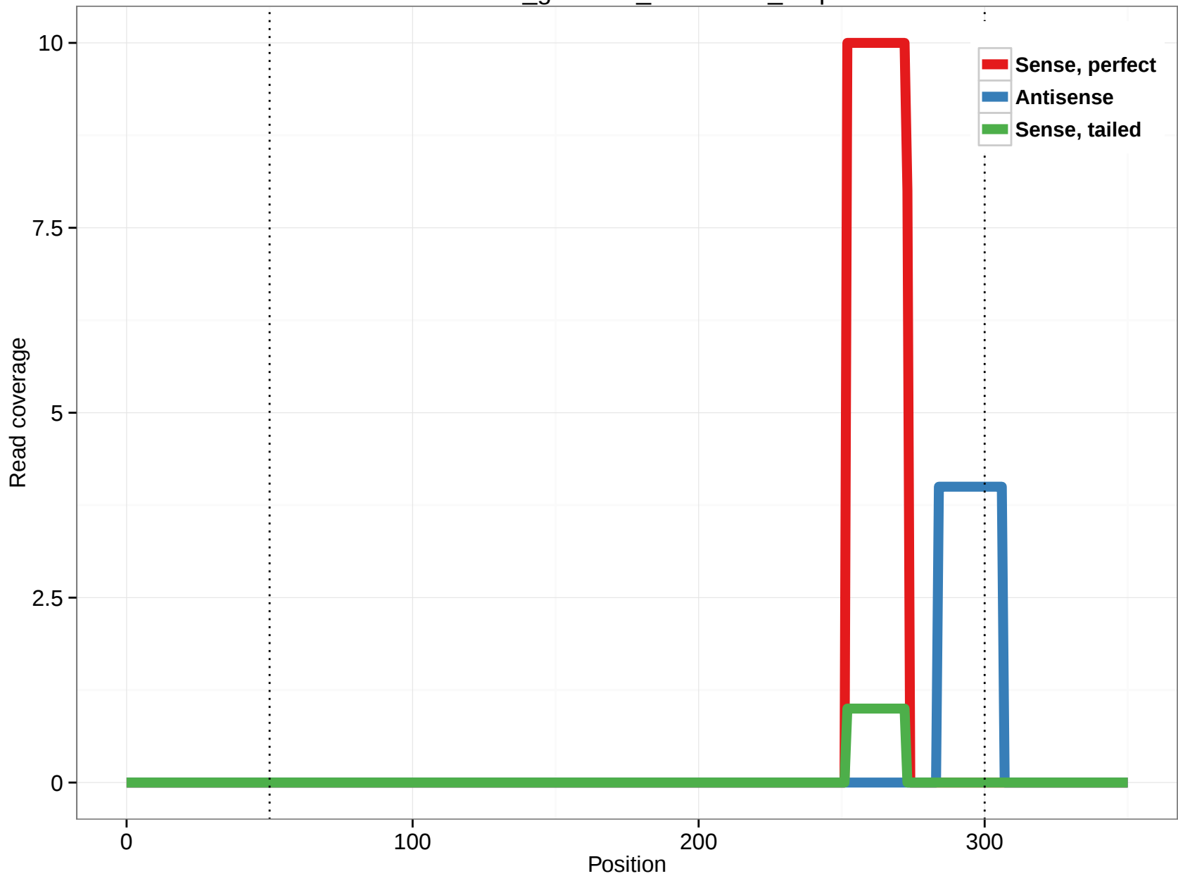
rheMac3_genscan_chr15.186_6.3p
