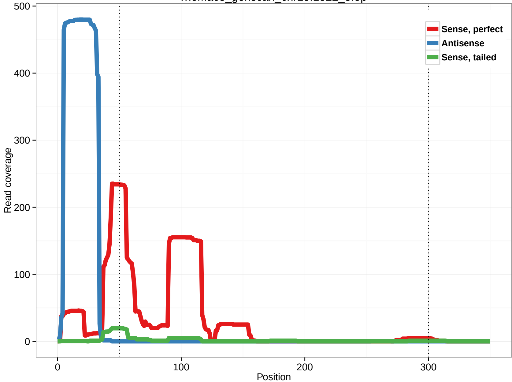
rheMac3_genscan_chr15.1822_8.5p
