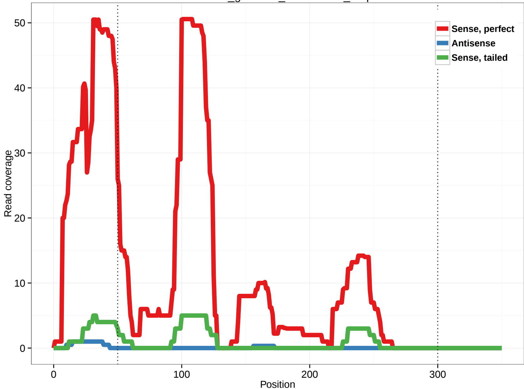
rheMac3_genscan_chr15.1822_5.5p
