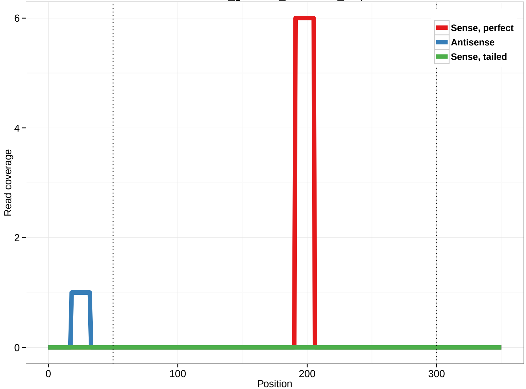
rheMac3_genscan_chr15.179_0.3p
