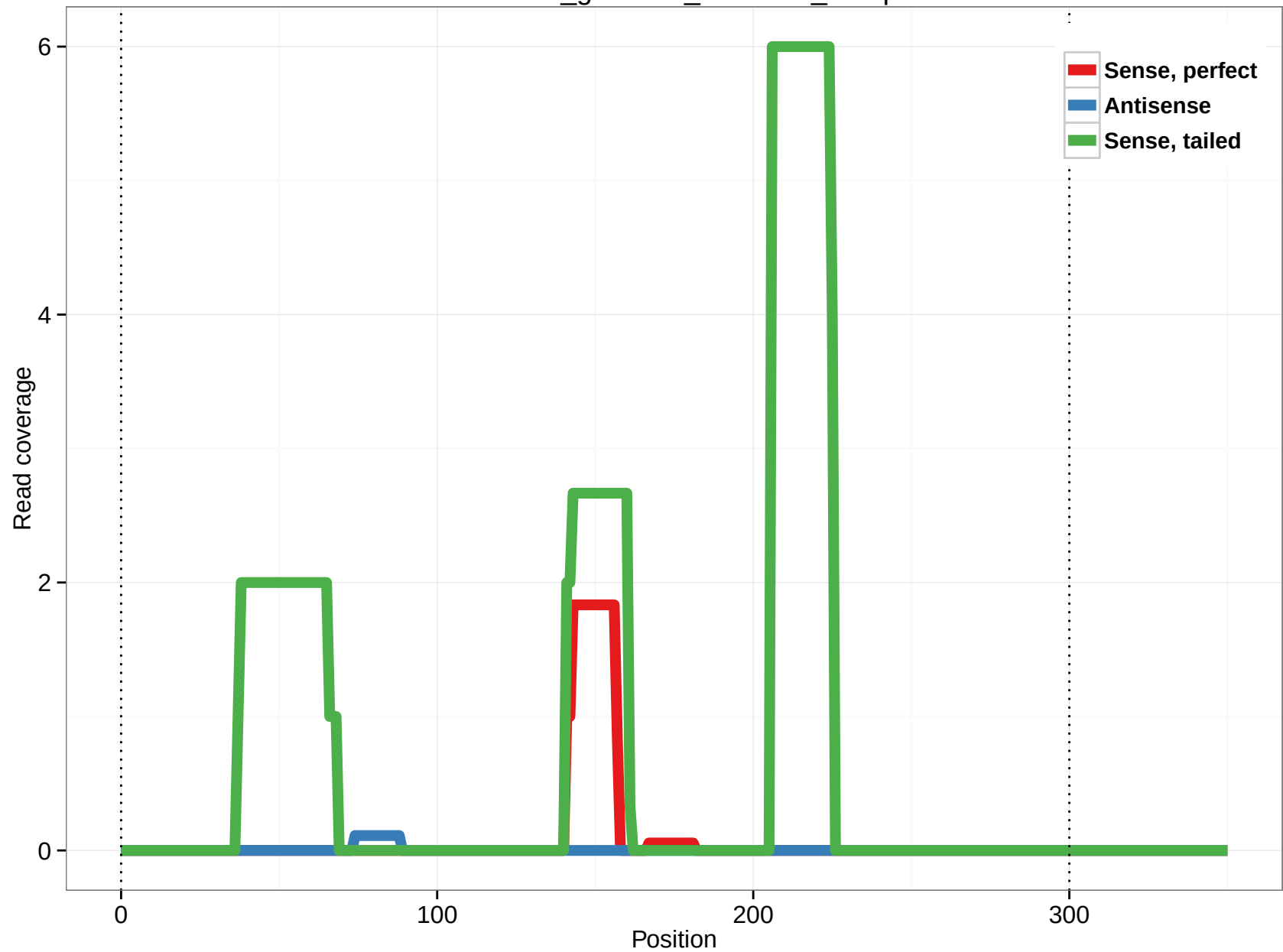
rheMac3_genscan_chr15.16_20.3p
