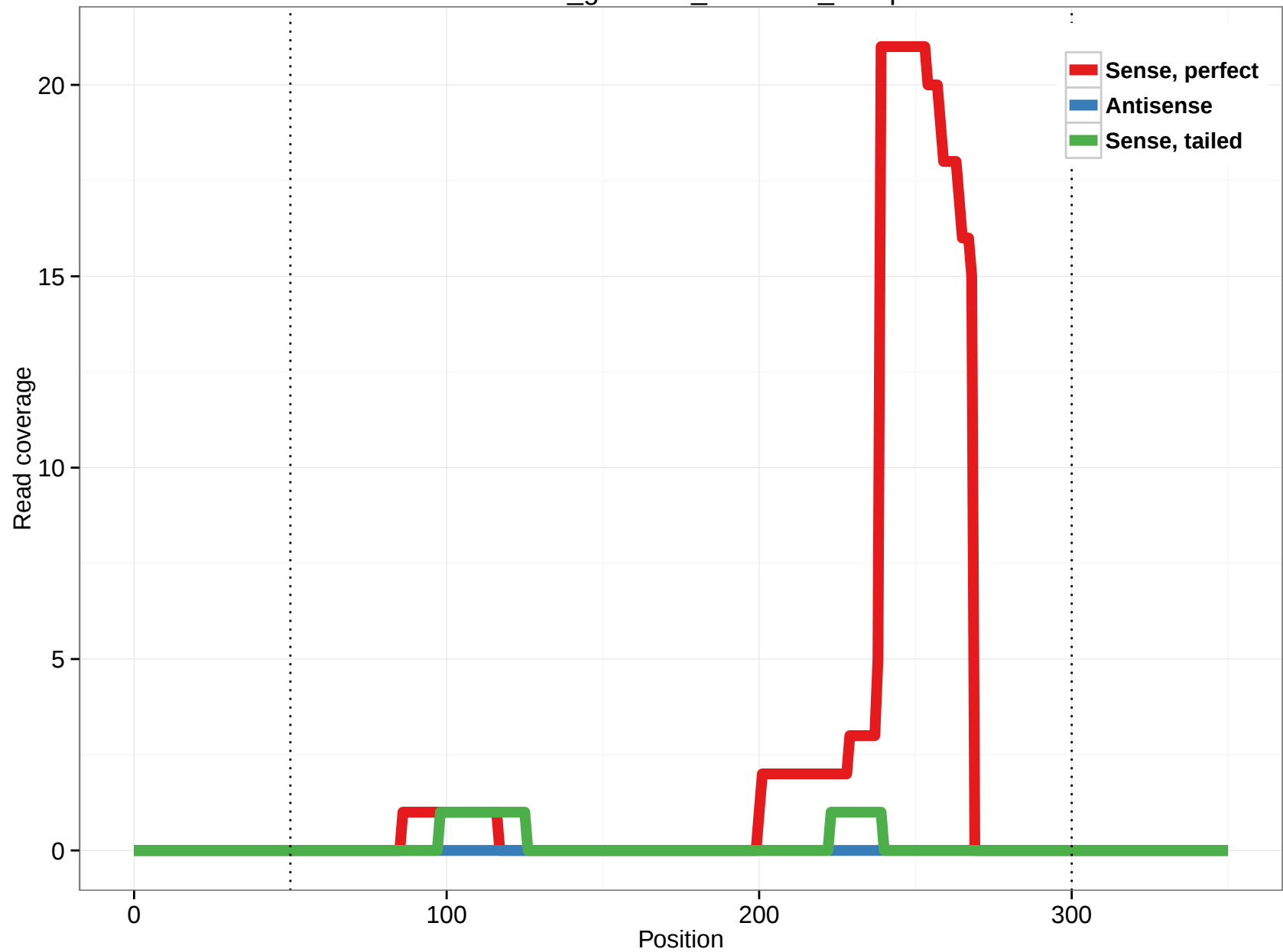
rheMac3_genscan_chr15.16_19.3p
