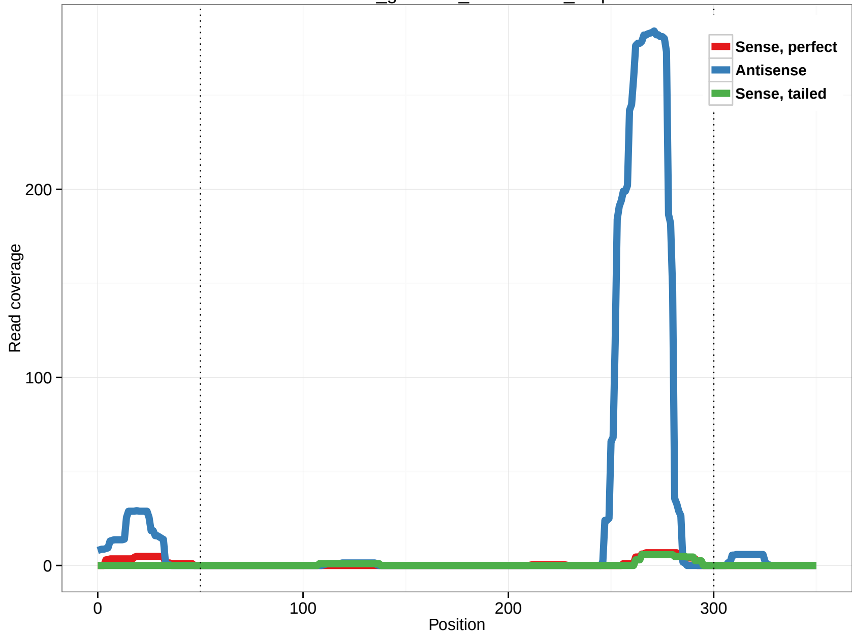
rheMac3_genscan_chr15.1689_5.3p
