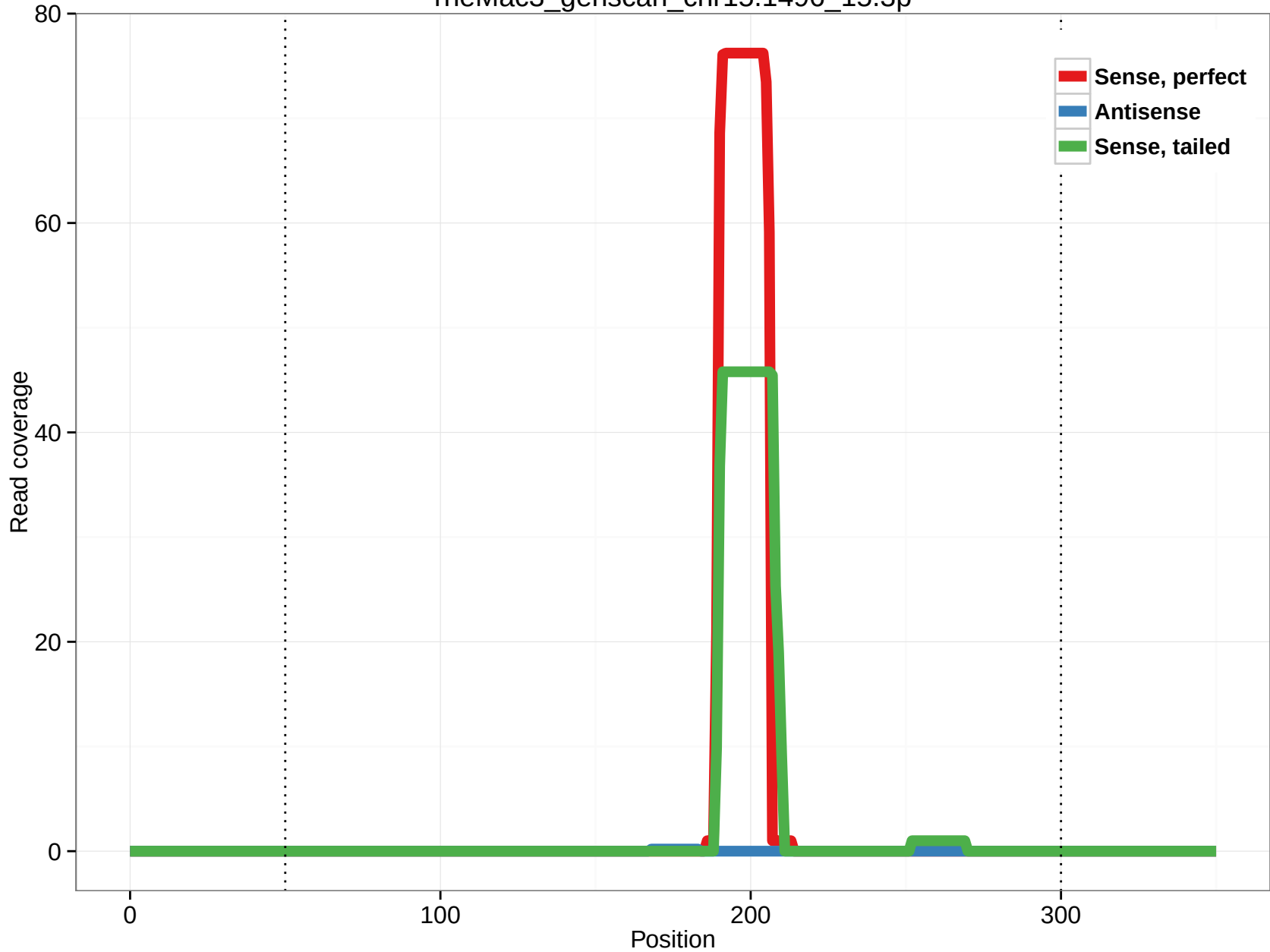
rheMac3_genscan_chr15.1496_15.3p
