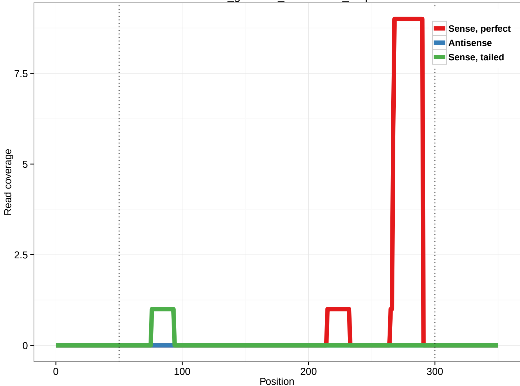
rheMac3_genscan_chr15.1490_8.3p
