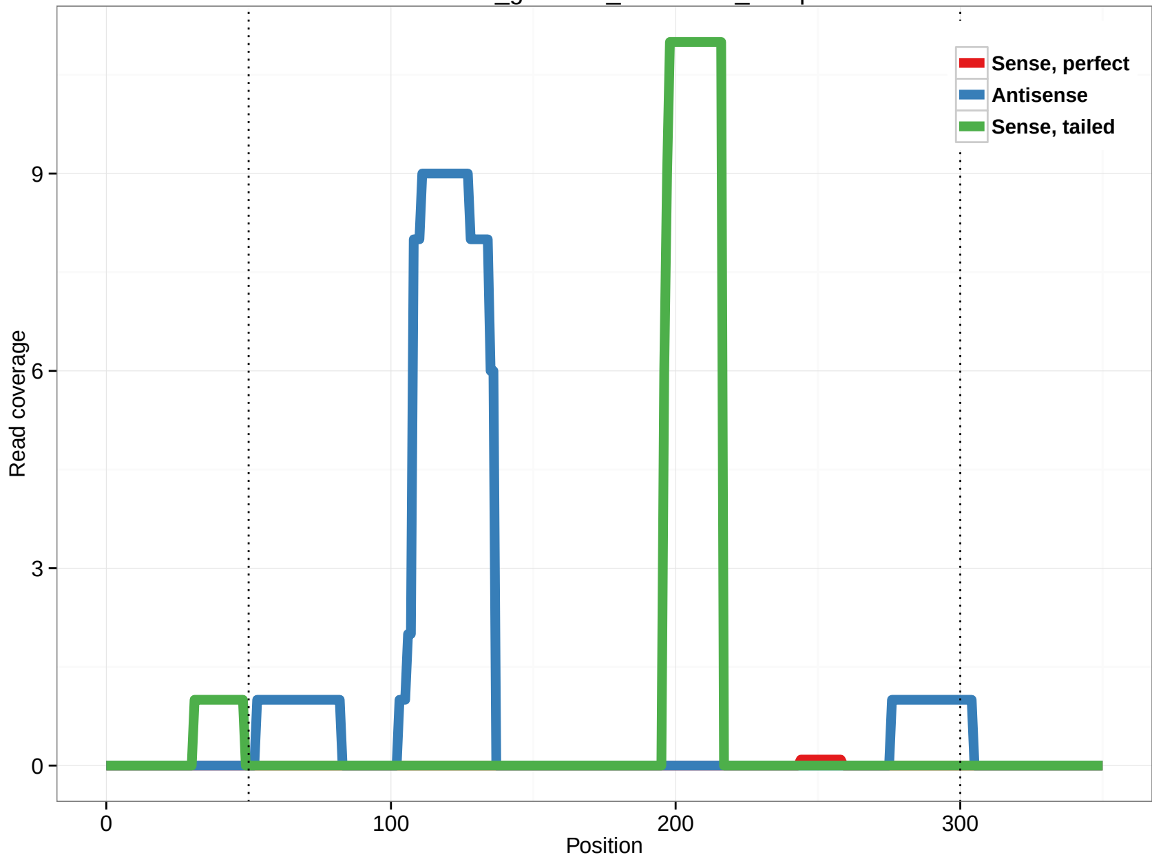
rheMac3_genscan_chr15.145_32.3p
