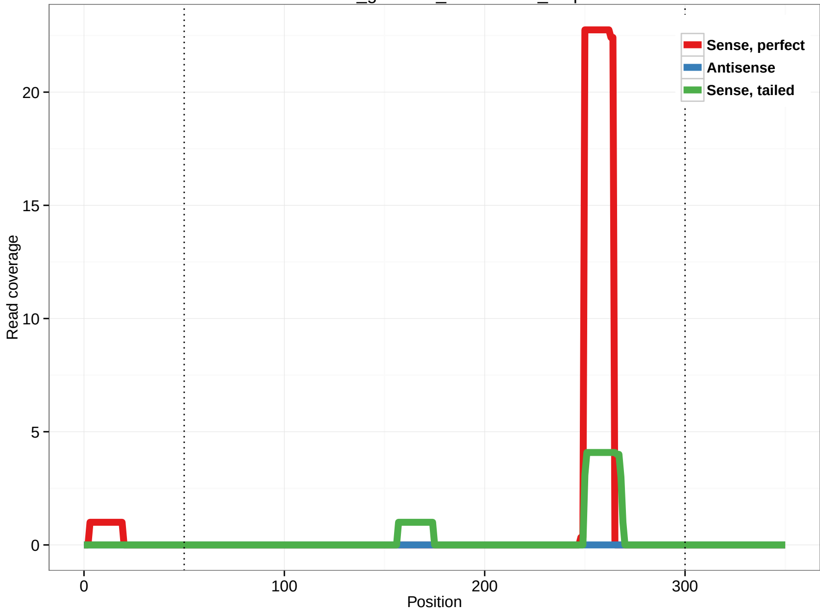
rheMac3_genscan_chr15.1458_2.5p
